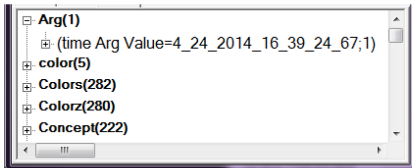
Fig. 57 Generate timestamp
