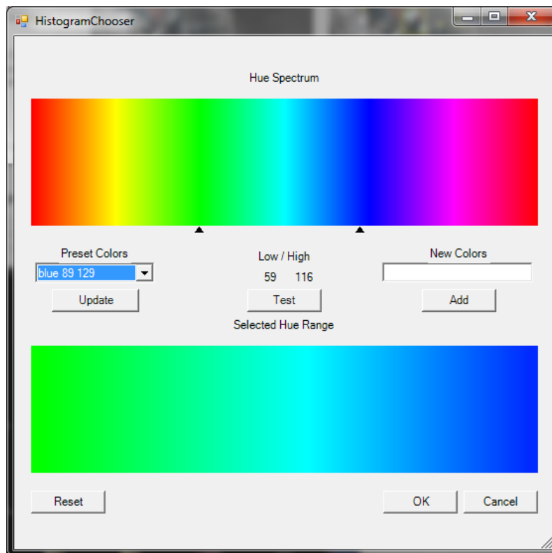
Fig. 97 Color HistogramChooser
