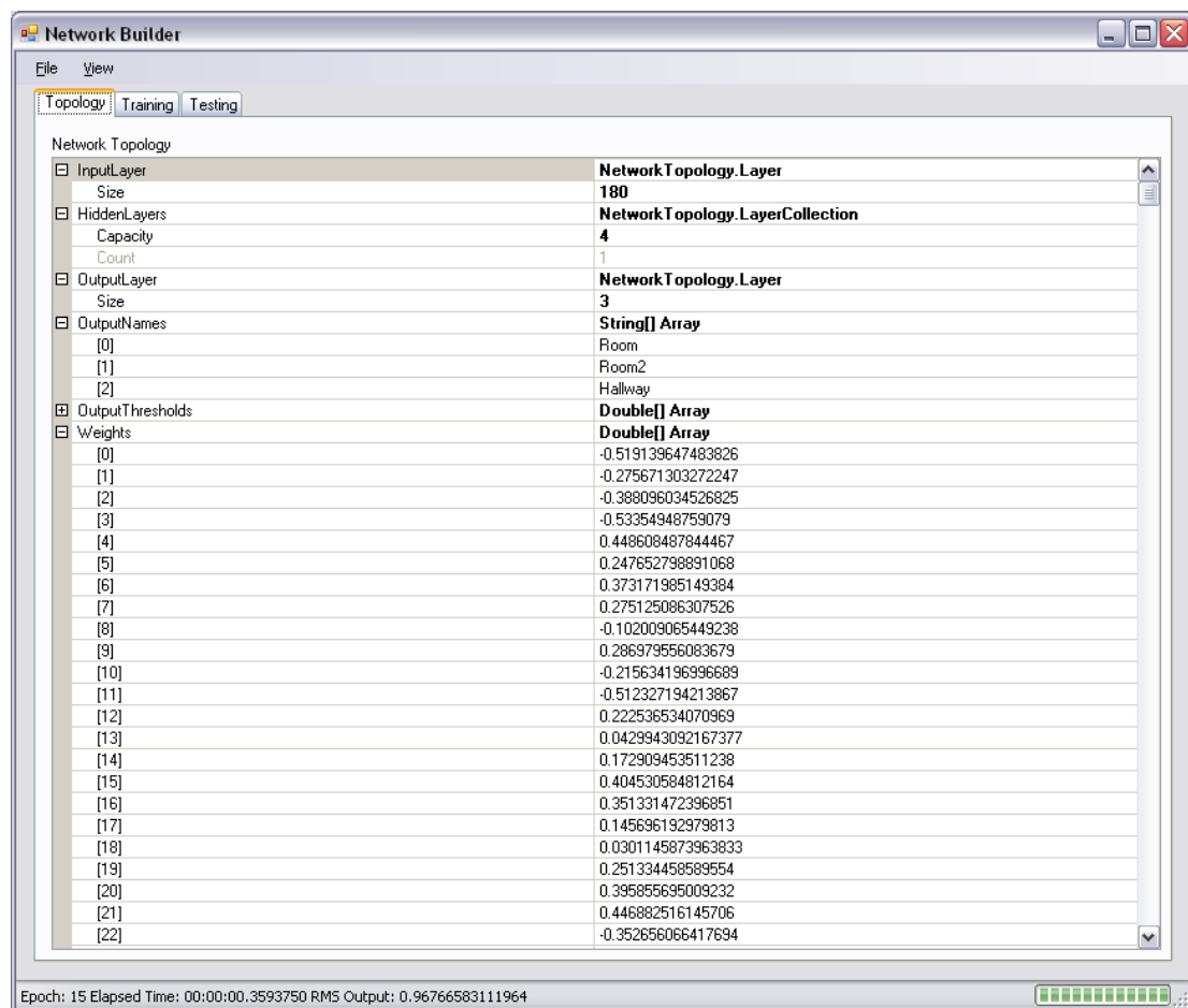
Fig. 143 Network Builder topology panel
