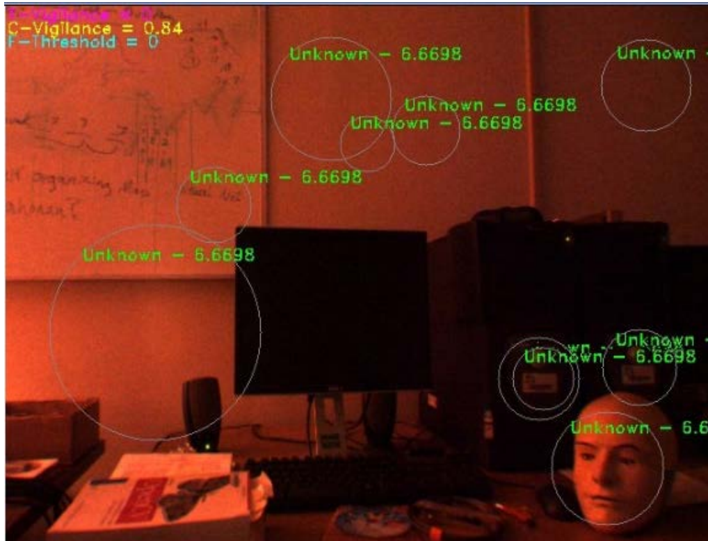
Fig. 85 False-positive faces
