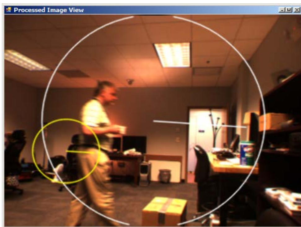
Fig. 105 Conventional view
