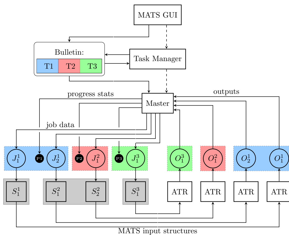
Figure 1.18: Architecture of MATS in distributed mode.
