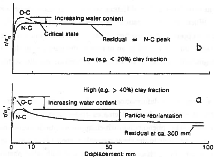
Fig. 2.8 Diagrammatic stress displacement curves (Ref. 3)
