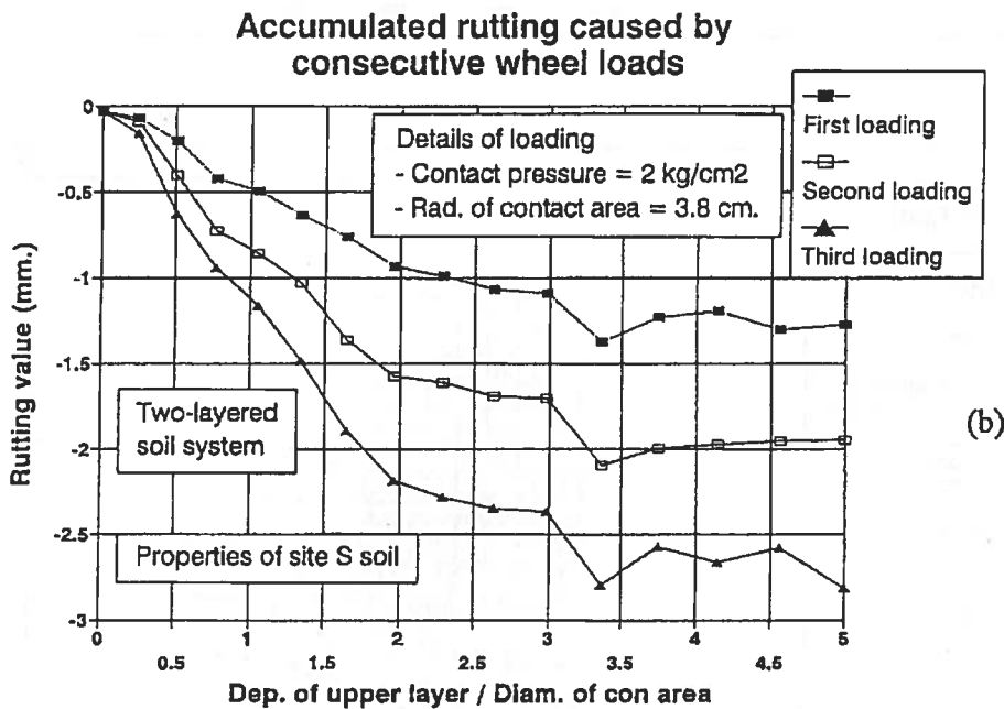
Fig. 6.20 Sinkage and rutting evaluation in a two-layered soil system (sub-system B2) with properties of site S material (a) Sinkage and rutting as a function of remolded layer depth. (b) Accumulated rutting values for consecutive loading of the same point as a function of remolded layer depth.
