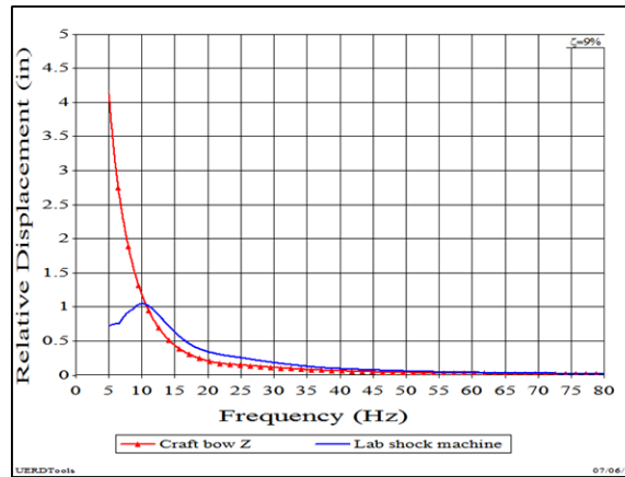
Figure C-4. DSRs for Wave Slam and Shock Machine Pulses
