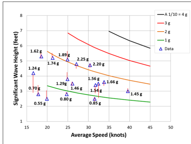
FigureB-5. A_{1/10} Trends for Category B Craft
