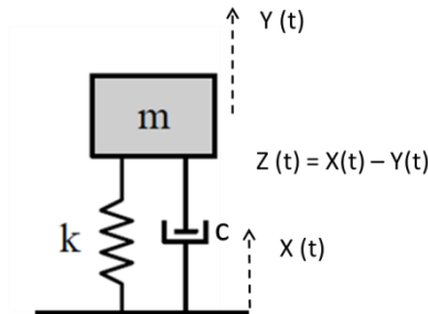
Figure C-1. Single-degree-of-freedom Mathematical Model
