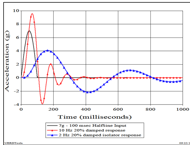
Figure D-2. Base Input and Shock Isolator Responses
