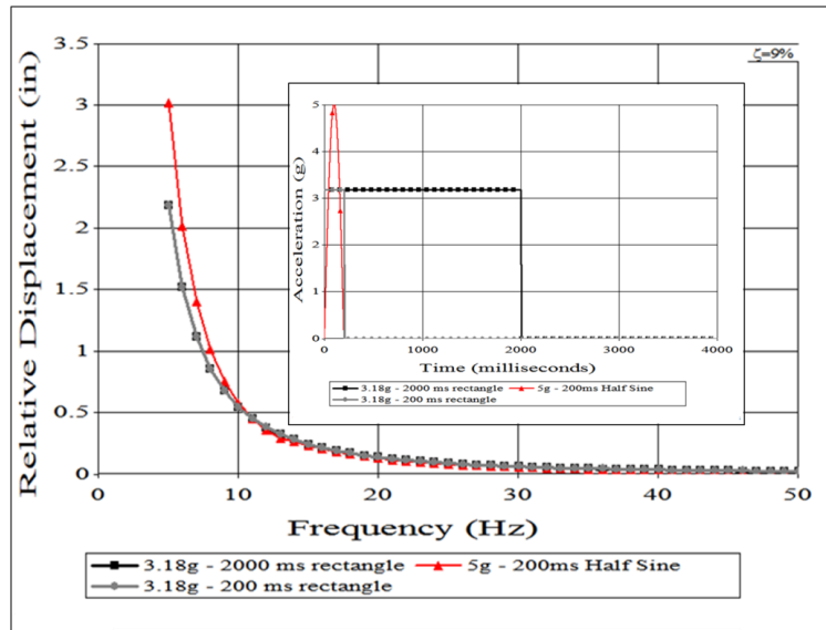
Figure 14. Relative Displacement SRS for Half-Sine and Square Pulses
