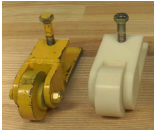
Figure 6: Original Versus 3D Printed Part 86
