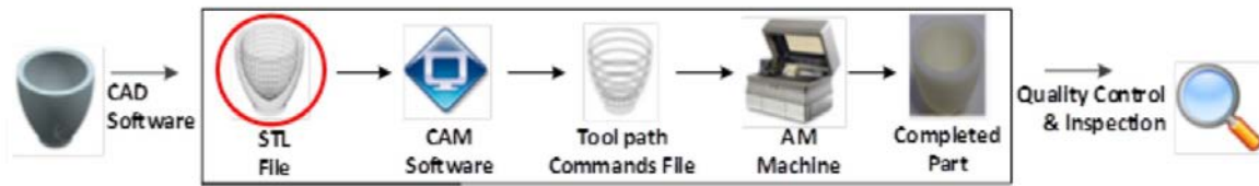
Figure 8: Additive Manufacturing Process Chain 103
