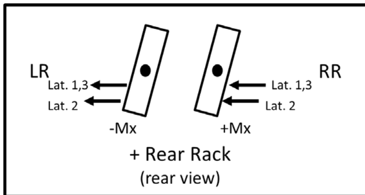
Figure C-4. Rear rack control channel actuator coupling and polarity.
