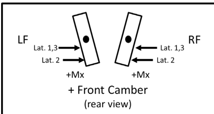
Figure C-5. Front camber control channel actuator coupling and polarity.
