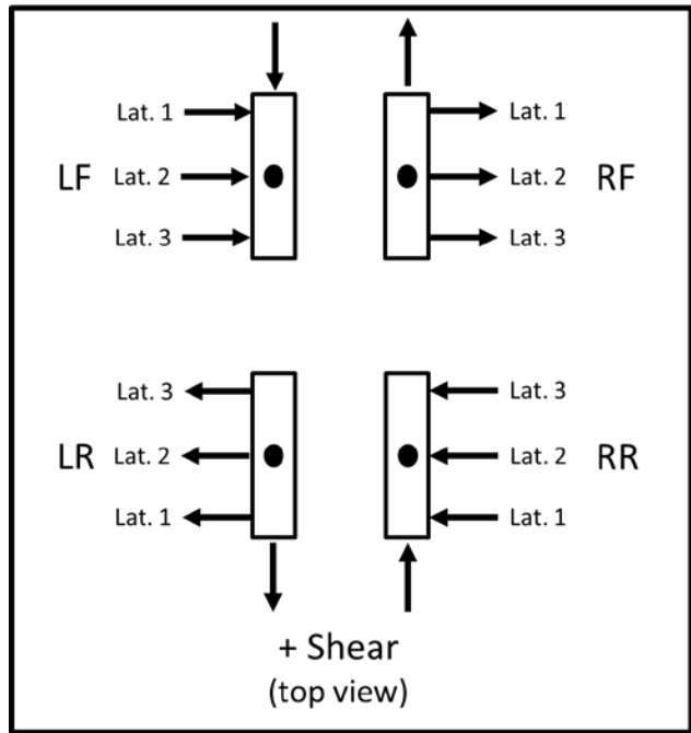
Figure C-11. Shear control channel actuator coupling and polarity.
