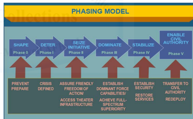
Figure 1: Phasing Model
