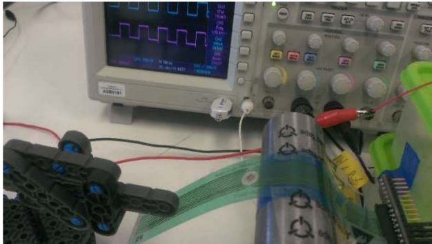
Fig. 6: 15mm Convex RoC Testing
