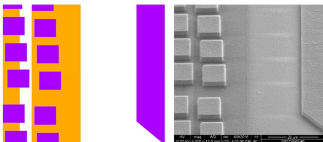
Fig. 10: FleX-IC Metal 4 Inspection Layout (L) and SEM (R)
