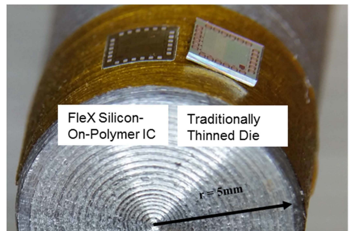
Fig. 2: FleX IC and Thinned Die on 5mm Radius Mandrel
