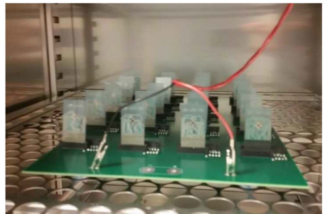
Fig. 8: FHE Test Configuration for HTOL and LTOL
