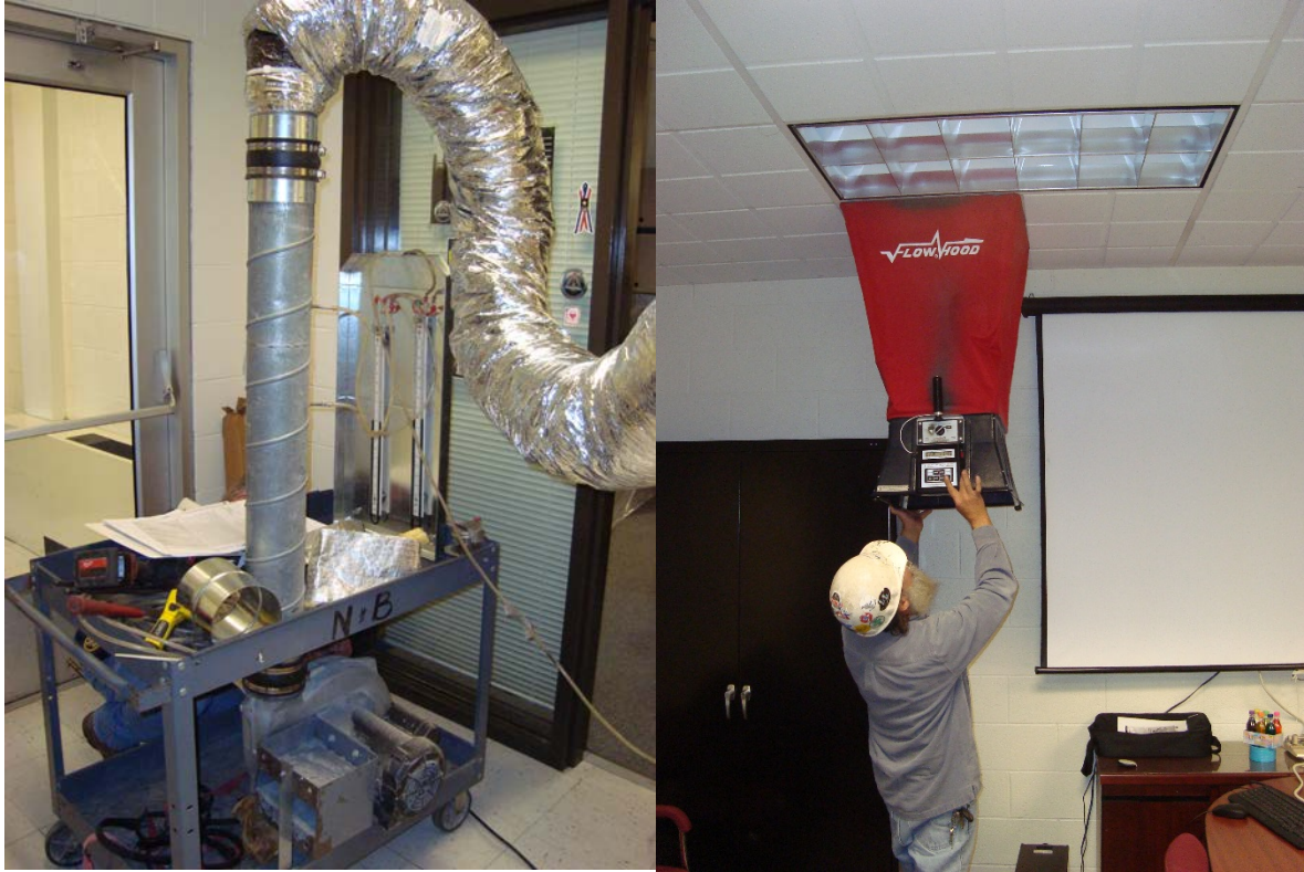
Figure 8. Duct Leakage Testing
