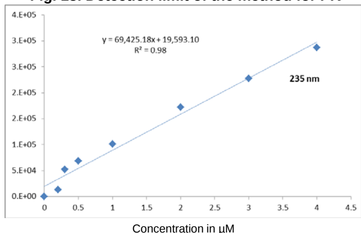
Fig. 13. Detection limit of the method for PK
