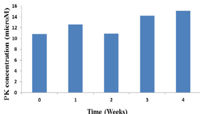
Fig. 15(b). PK Stability study at 37°C in PEG400
