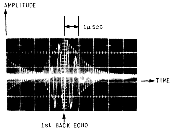
Figure 3. ULTRASONIC DUAL FREQUENCY TESTING
