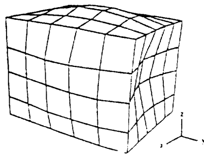
Mode 1 (658.37 Hz)
