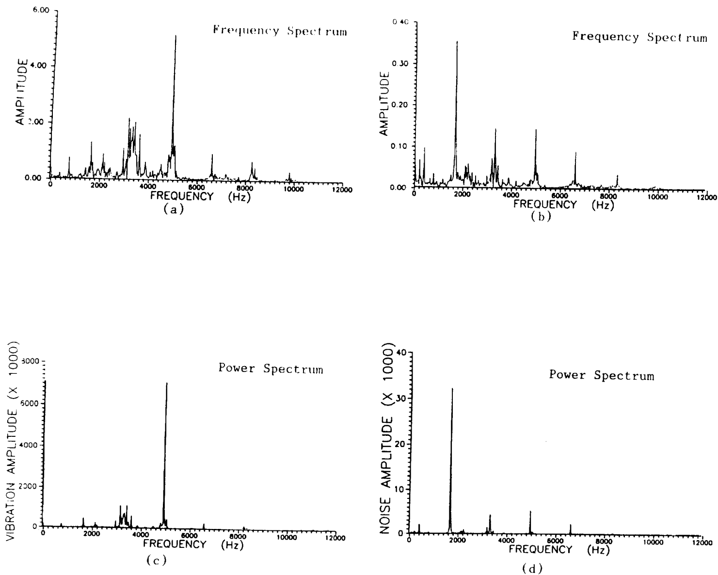
Figure 7.9 Frequency spectrum for (a) vibration, (b) noise from microphone no. 2, and power spectrum for (c) vibration, (d) noise from microphone no. 2, at the operating speed of 4,000 rpm.
