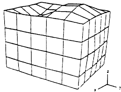
Mode 2 (1048.56 Hz)
