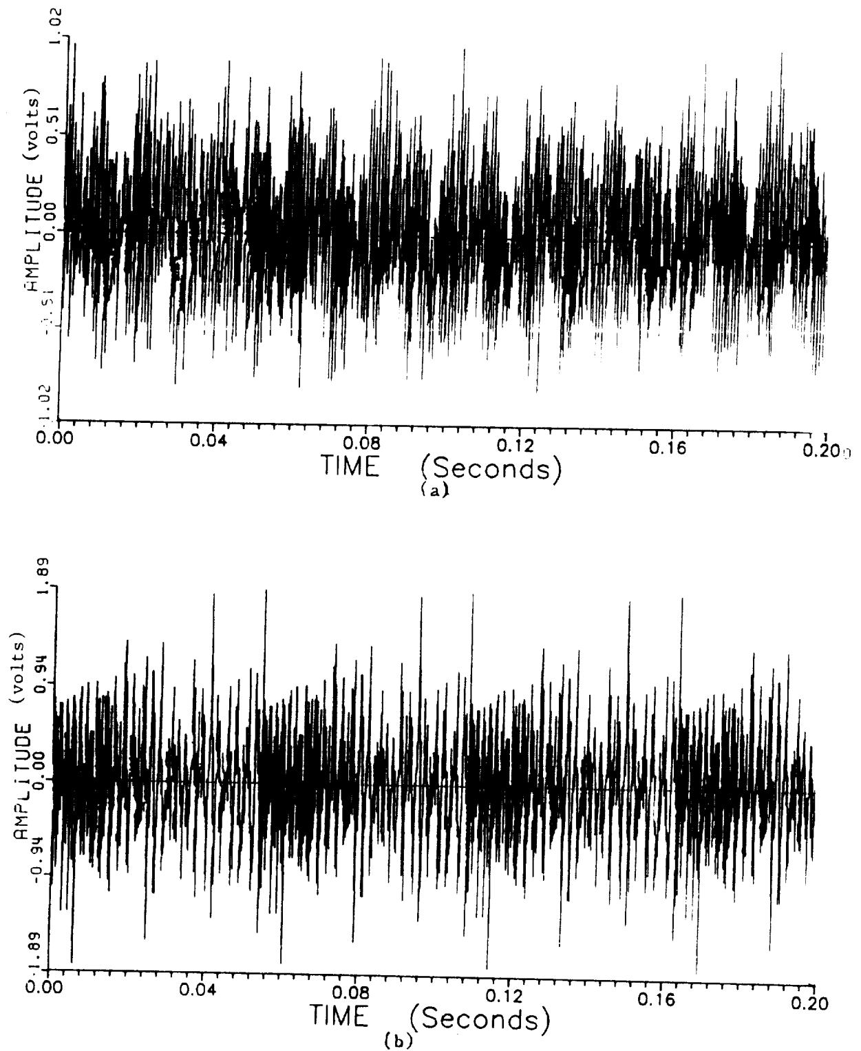
Figure 7.22 Time noise signal from (a) experimental noise data, and (b) predicted noise results from microphone no. 2 at the operating speed of 3,000 rpm.
