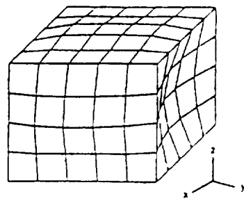
Mode 1 (658 Hz)
