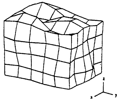
Mode 8 (2961.71 Hz)
