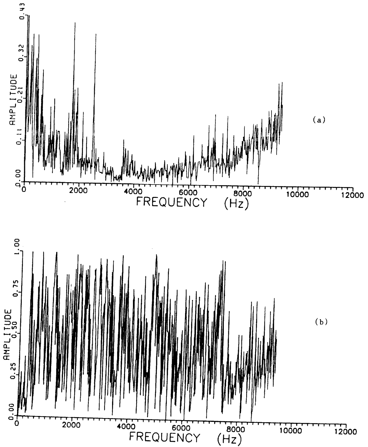
Figure 7.6 (a) Transfer function and (b) coherence function, between noise (microphone no. 2) and vibration at the operating speed of 3,000 rpm
