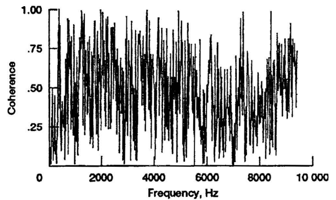
(b) Coherence function.
