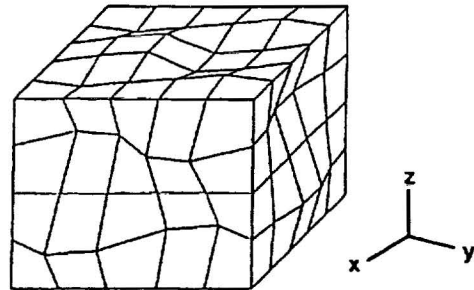
Mode: 4 Frequency = 2051
