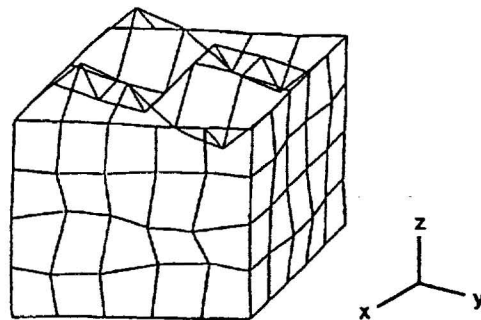
Mode: 8 Frequency = 3012
