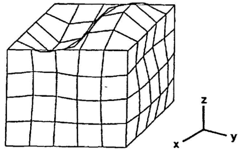
Mode: 2 Frequency = 1006
