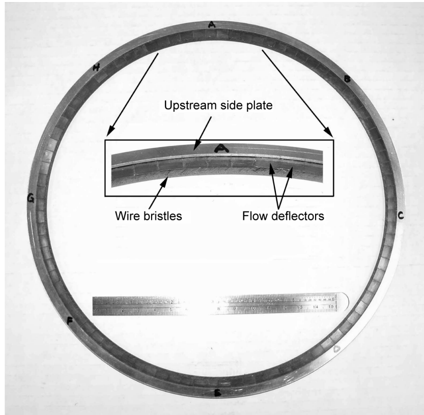
Figure 5.—Brush seal with flow deflector.
