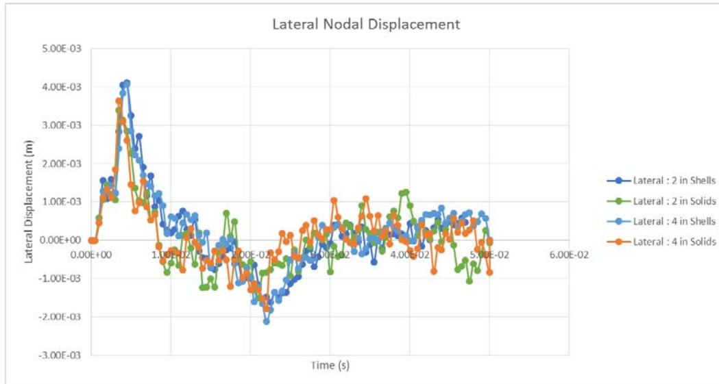
Fig. 5 Lateral nodal displacement for solid and shell surrogate models
