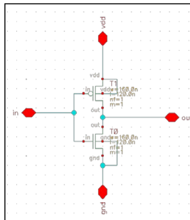
Figure 4. Inverter schematic.
