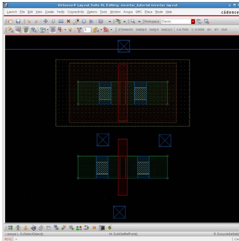
Figure 10. Updated layout with components moved into location.
