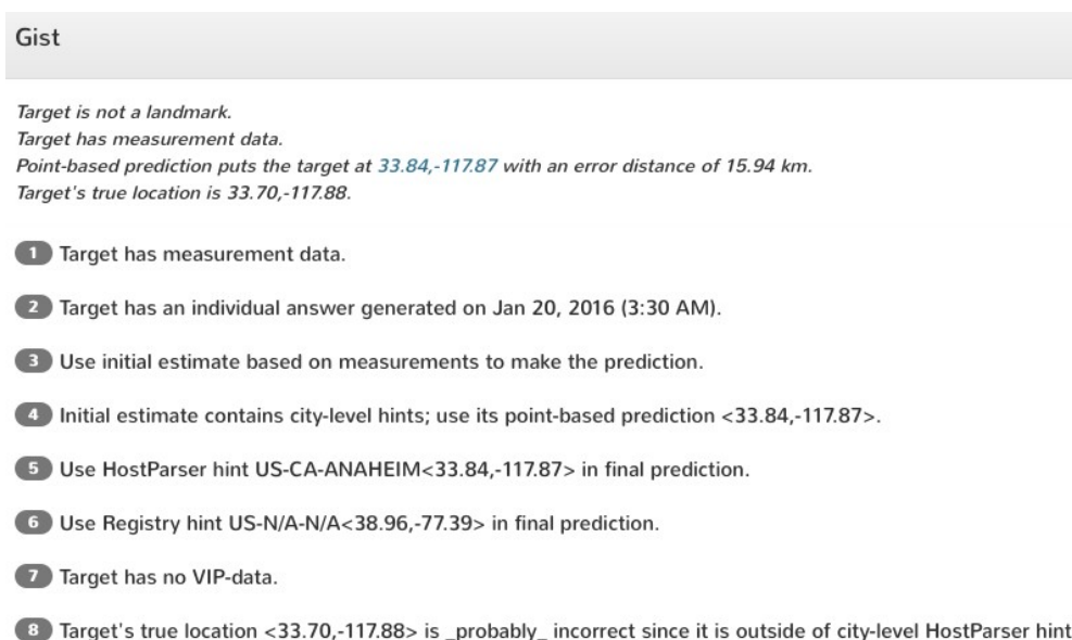
Figure 4: Alidade's prediction for a target highlighting (in the last step of the gist) that the ground truth location of the target may be incorrect. The ground truth location is contained in the area formed by intersecting direct measurements, but not contained within the feasible region of the prediction.
