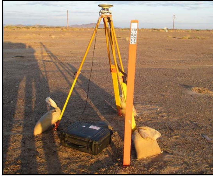
Figure B-2. GPS reference station.
