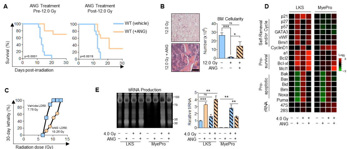
Figure 4. ANG enhances radioprotection and radioresistance. (A) Survival of WT mice treated with ANG daily for three successive days 24 h prior or post-12.0 Gy. (B) H&E and BM cellularity of femurs of WT mice treated with ANG daily for three successive days 24 h post-12.0 Gy (n=6). Scale bar = 100 \mu m. (C) LD50 of mice treated with ANG daily for three successive days beginning 24 h post-TBI (n=8). (D-E) qRT-PCR analysis of pro-self-renewal, pro-survival, pro-apoptotic, and rRNA transcripts (D, n=6), and tRNA production (E, n=3) in LKS or MyePro sorted from irradiated mice (4.0 Gy) and treated with 300 ng/ml ANG.
