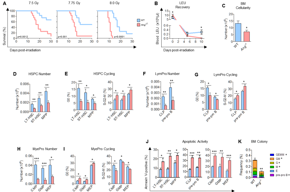
Fig. 1. Increased sensitivity of Ang^{-/-} mice to \gamma -irradiation. (A) Kaplan-Meier survival curves of WT or Ang^{-/-} mice subjected to 7.5 Gy (left), 7.75 Gy (middle), or 8.0 Gy (right) radiation (n=12). (B) Blood leukocyte recovery in WT or Ang^{-/-} mice treated with 8.0 Gy (n=10). (C-J) BM cellularity (C), HSPC number per femur (D), HSPC cycling (E), LymPro number per femur (F), LymPro cycling (G), MyePro number per femur (H), MyePro cycling (I), apoptotic activity (J), and colony formation (K) of WT or Ang^{-/-} mice treated with 4.0 Gy TBI (n=6). Animals were sacrificed and analyzed on day 7 post-irradiation.
