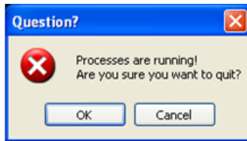
Figure 5. Exit pop-up.
