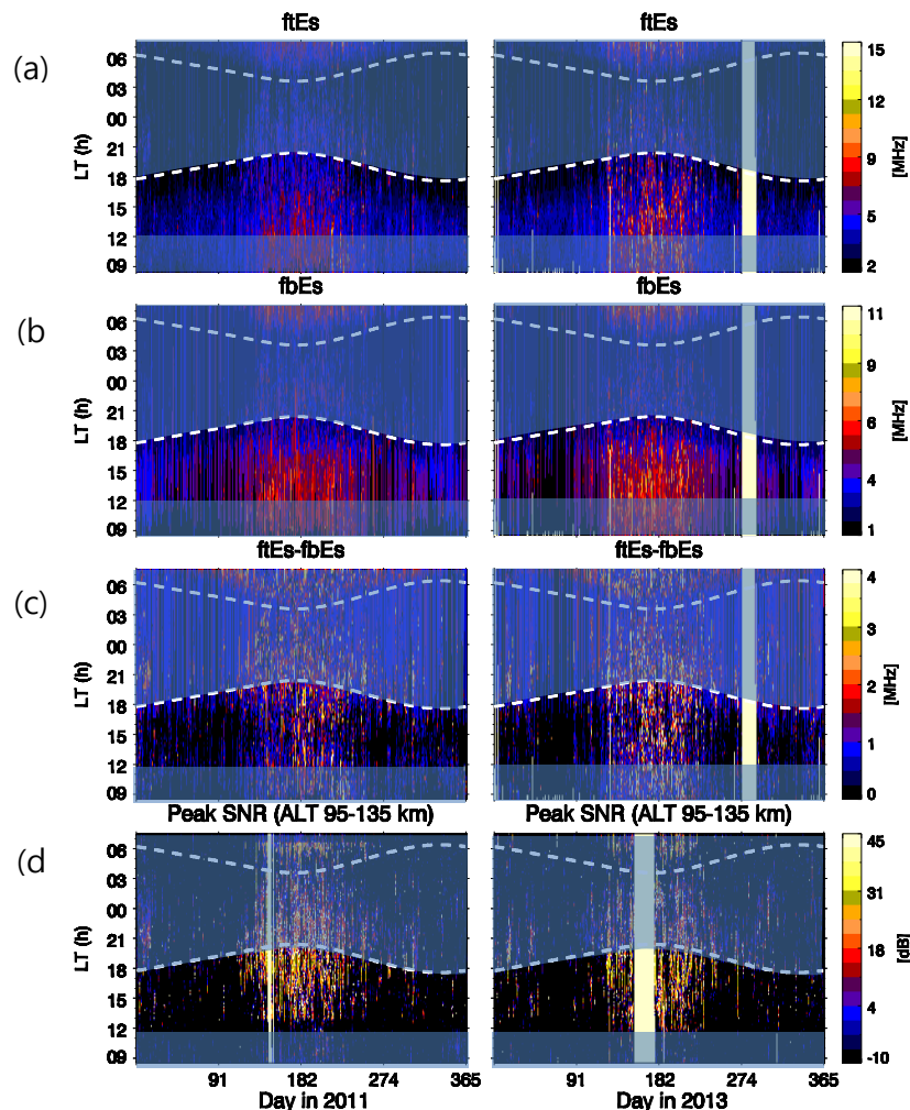
Figure 15. (a-c) Seasonal and local time distributions of the three E_s parameters ( f_iE_s , f_bE_s and f_iE_s - f_bE_s ) observed from Icheon ionosonde and (d) peak SNR of E -region FAIs observed from Daejeon VHF radar in 2011 and 2013.
