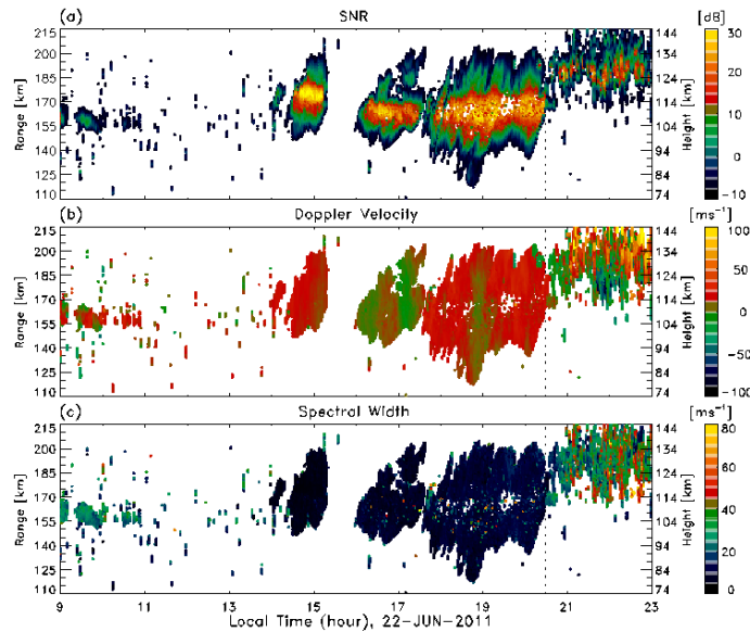
Figure 11. Range-time variations of (a) signal-to-noise ratio (SNR), (b) Doppler velocity and (c) spectral width of the E -region irregularities observed on 22 June 2011. Vertical dotted line represents sunset time in the E region.
