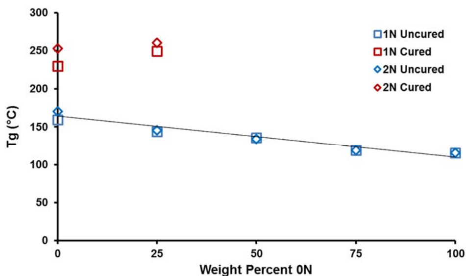
Figure 12. The dependence of uncured and cured T_g as a function of 0N mix ratio in blends with 1N and 2N, respectively. The cured T_g s of the systems containing more than 25 percent by weight of 0N could not be identified.
