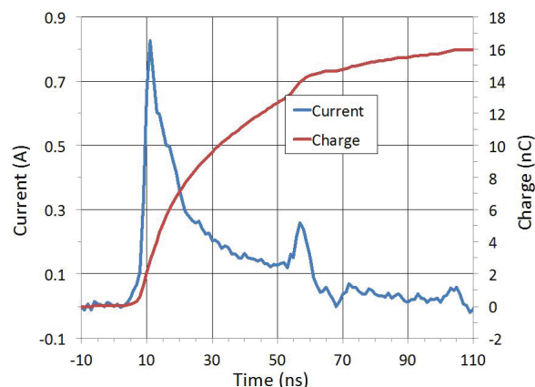
Figure 3. Helium current and integrated charge versus time at the target measured with the fast Faraday cup. The sharp peak in the current measurement shows the beam pulse compression from 1 \mu s to a few ns. The full temporal extension of the pulse is ~50 ns with a ~1 ns rise time. The second peak around 56 ns is formed by late arriving ions with slightly lower energies due to ringing in one of the acceleration voltage pulses.
