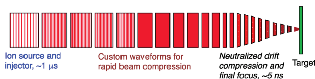
Figure 2. Beam compression in NDCX-II.
