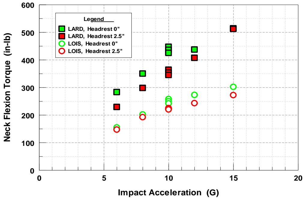
Figure 36. Neck Flexion Torque as a Function of Impact Accel. and Headrest Position With Reclined Seat
