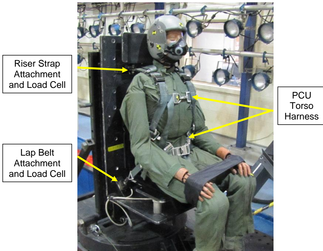
Figure 5. PCU Torso Hanes on the LARD Manikin on HIA Sled
