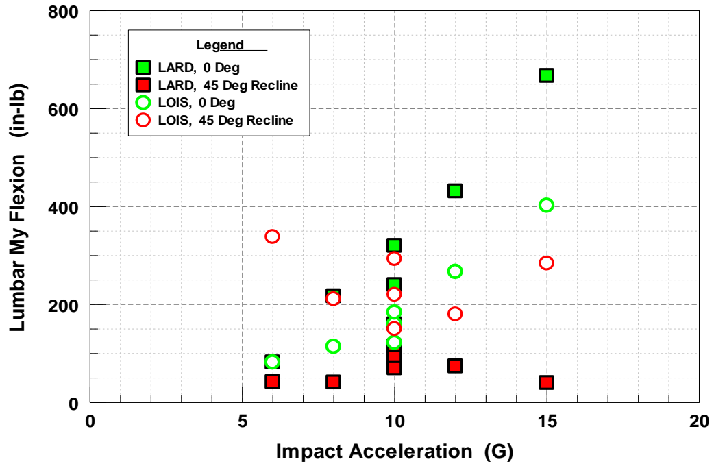
Figure 32. Lumbar My Flexion as a Function of Impact Accel. and Seat Tilt Variation
