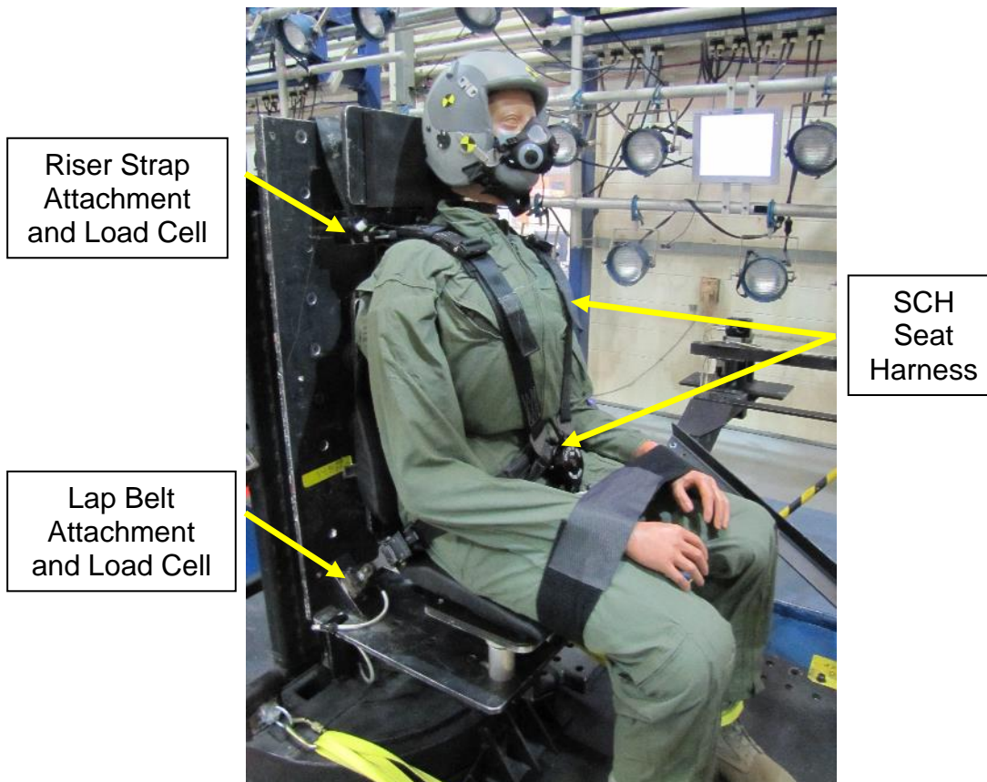
Figure 6. SCH Seat-Mounted Hanes on the LARD Manikin on HIA Sled
