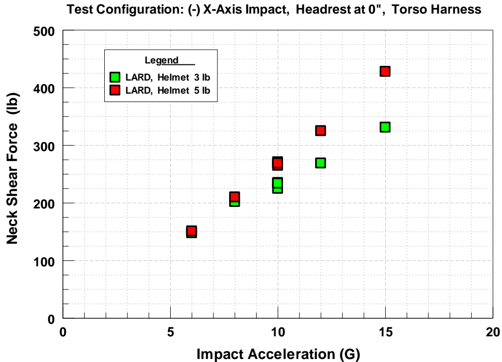
Figure 19. Neck Shear Force as a Function of Impact Acceleration and Helmet Weight
