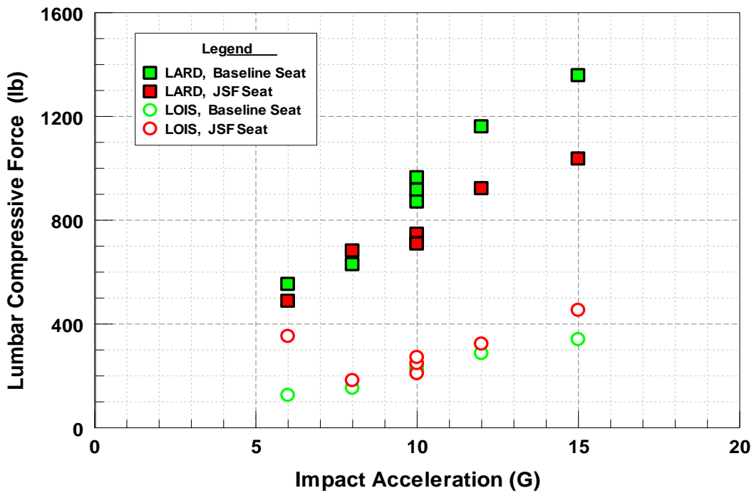
Figure 26. Lumbar Compression as a Function of Impact Accel. and Seat Configuration
