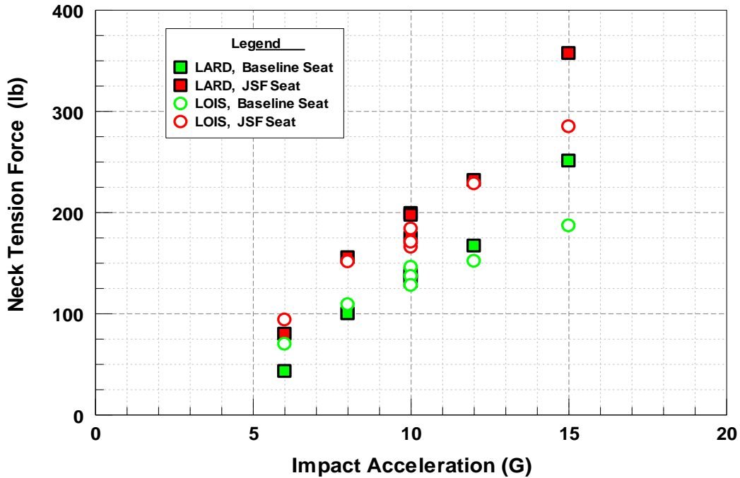
Test Set-up: (-) X-Axis Impact, Headrest 0"/2.5", Helmet 55P/JSF, Harness Torso/Seat
