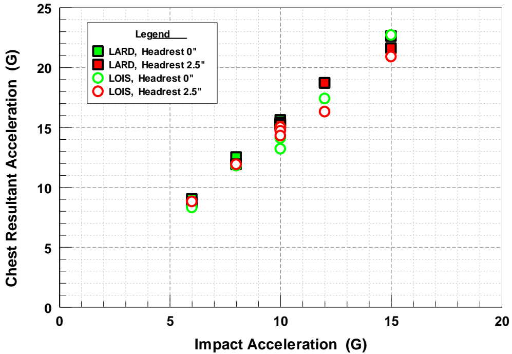
Figure 37. Resultant Chest Accel. as a Function of Impact Accel. and Headrest Position With Reclined Seat
