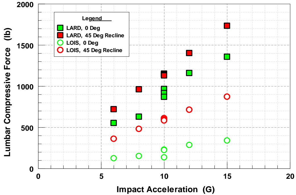
Figure 31. Lumbar Compression as a Function of Impact Accel. and Seat Tilt Variation
