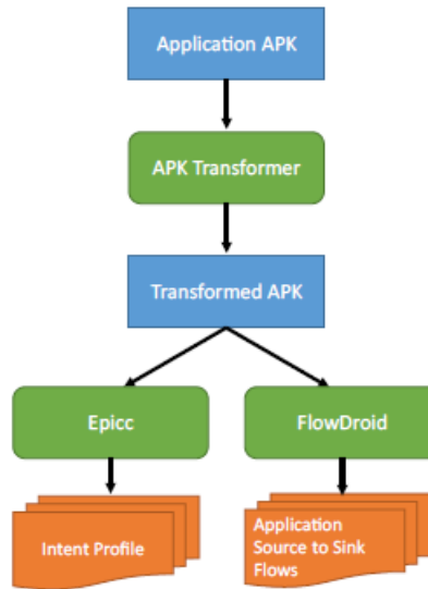
Figure 1.1: Overview of DidFail Phase 1
