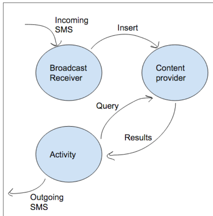
Figure 4.6: Flows in Example App 1 for Content Providers
