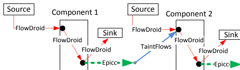
Figure 1.2: Data Flow Taint Tracking
