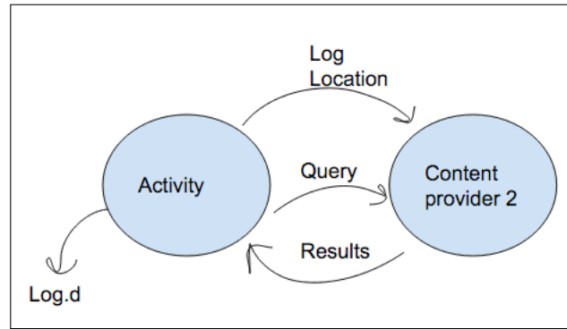
Figure 4.9: Flows in Example App 2 for Content Providers
