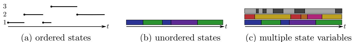
Figure 3: Example continuous-time Markov process samples (trajectories)
