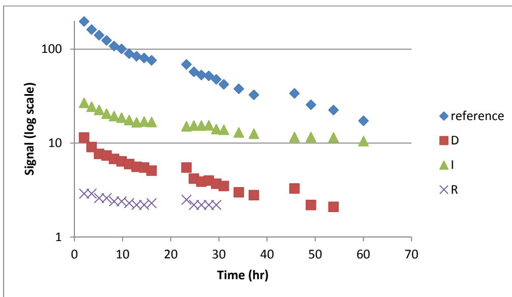
Figure 7. Decrease in signal for GD for the reference material relative to the treated materials 20130509D, I, and R, using an agent challenge of 10 \mu\text{g} ( 0.18 \text{ g/m}^2 ). The signal is plotted on a log scale. The trace indicates that breakthrough of the agent isn't occurring.
