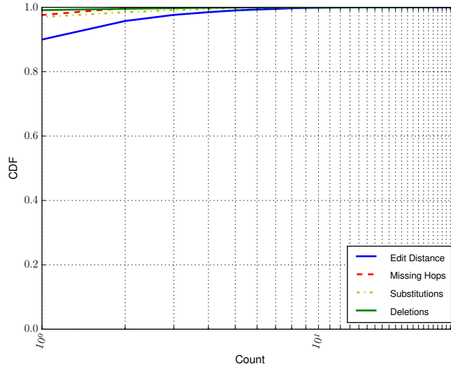
Figure 4.3. Edit Distance of Two Different CAIDA Scans Separated by 15 Hours.
