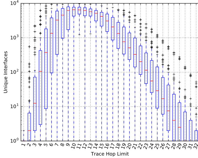
Figure 4.7. Distribution of Interfaces Discovered as a Function of Hop Limit.
