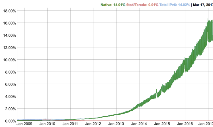
Figure 1.1. Percentage of Users Accessing Google over IPv6 (March 2017). Source: [27].
