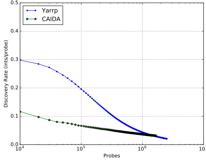
Figure 4.6. Discovery Rate of Yarrp6 versus CAIDA as a Function of Probes Sent.
