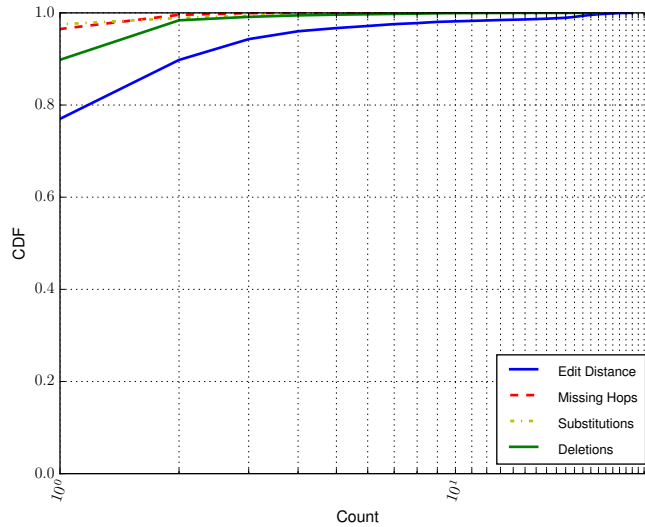
Figure 4.2. Edit Distance of Yarrp6 versus CAIDA.
