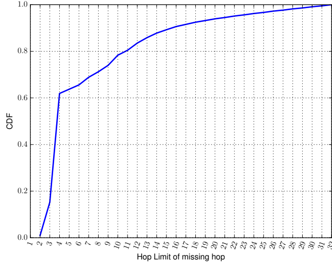
Figure 4.4. CDF of Missing Hops by TTL in Yarrp6 ICMPv6 Scan Results.
