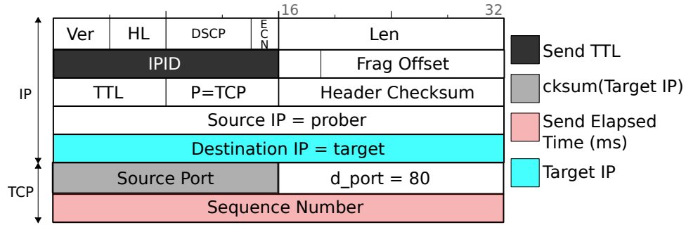
Figure 2.2. Yarrp Encoding of IPv4 and TCP Header. Source: [16].
