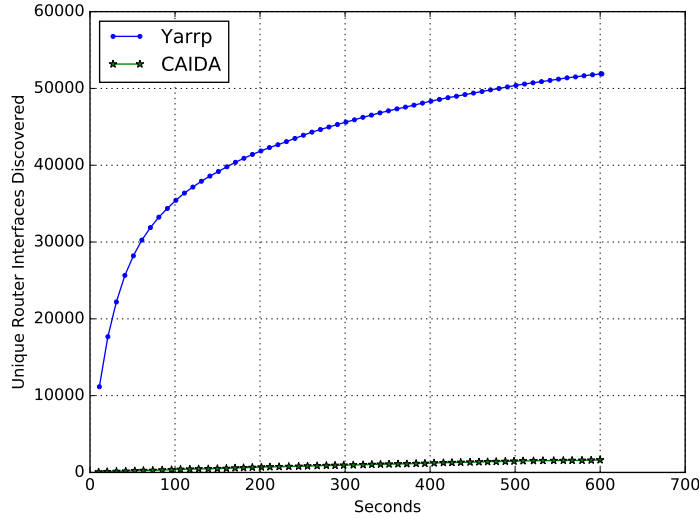
Figure 4.5. Discovery Rate of Yarrp6 versus CAIDA as a Function of Time.
