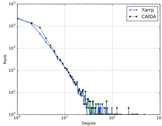
Figure 4.1. Degree Distribution of Yarrp6 versus CAIDA.
