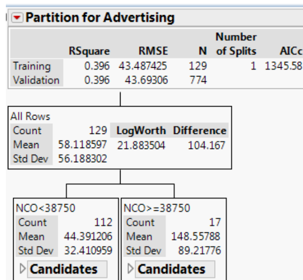
Figure 63. Parent and First Child Node of Partition Tree for Advertising
