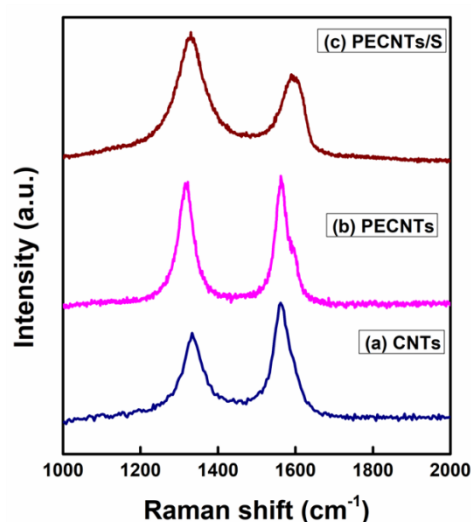
Fig 2. Raman spectra of (a) CNTs (b) PECNTs (c) PECNs/S
