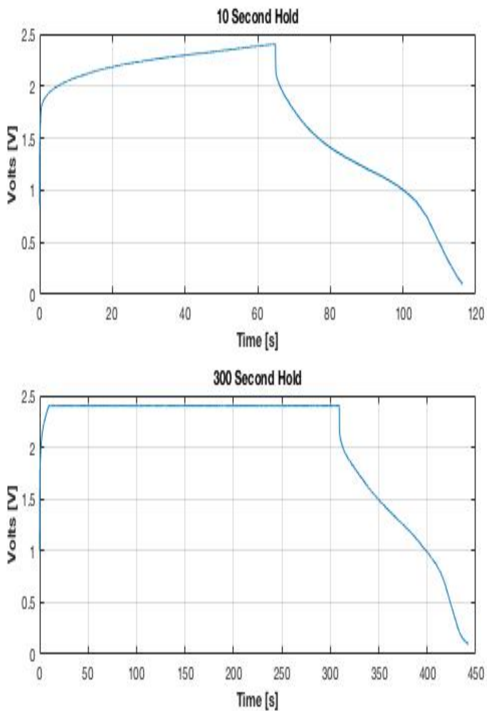
Figure 45. PC + DI/NaCl Solution for FHS Testing
