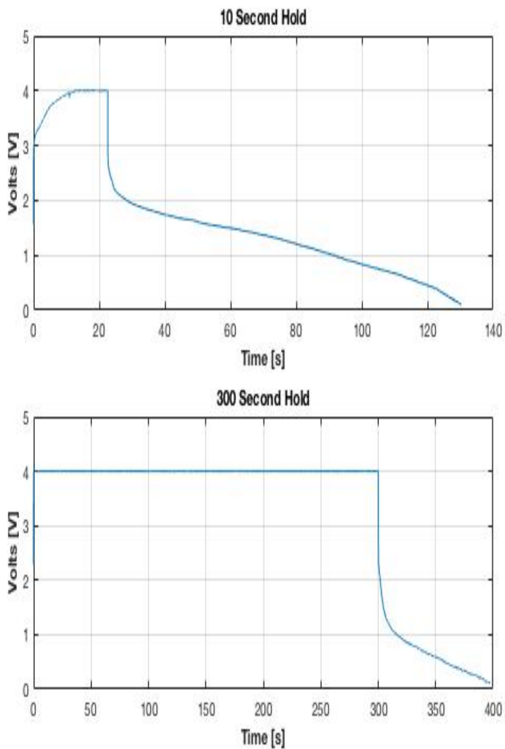
Figure 29. PC + DI/NaCl Solution for FHS Testing
