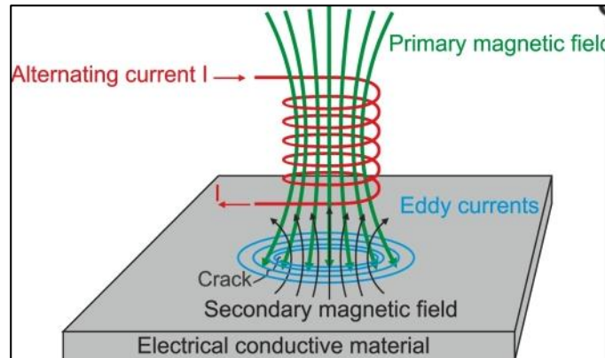
Figure 10. Sketch of ECT Physical Principles. Source: García-Martín, Gómez-Gil, and Vázquez-Sánchez (2011).
