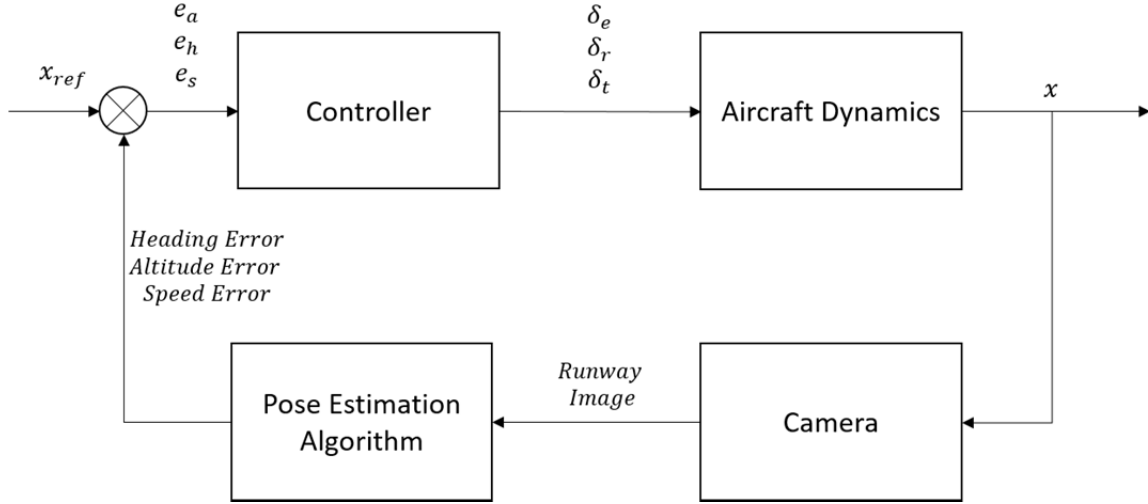
Figure 2. Vision-Based Landing Control System
