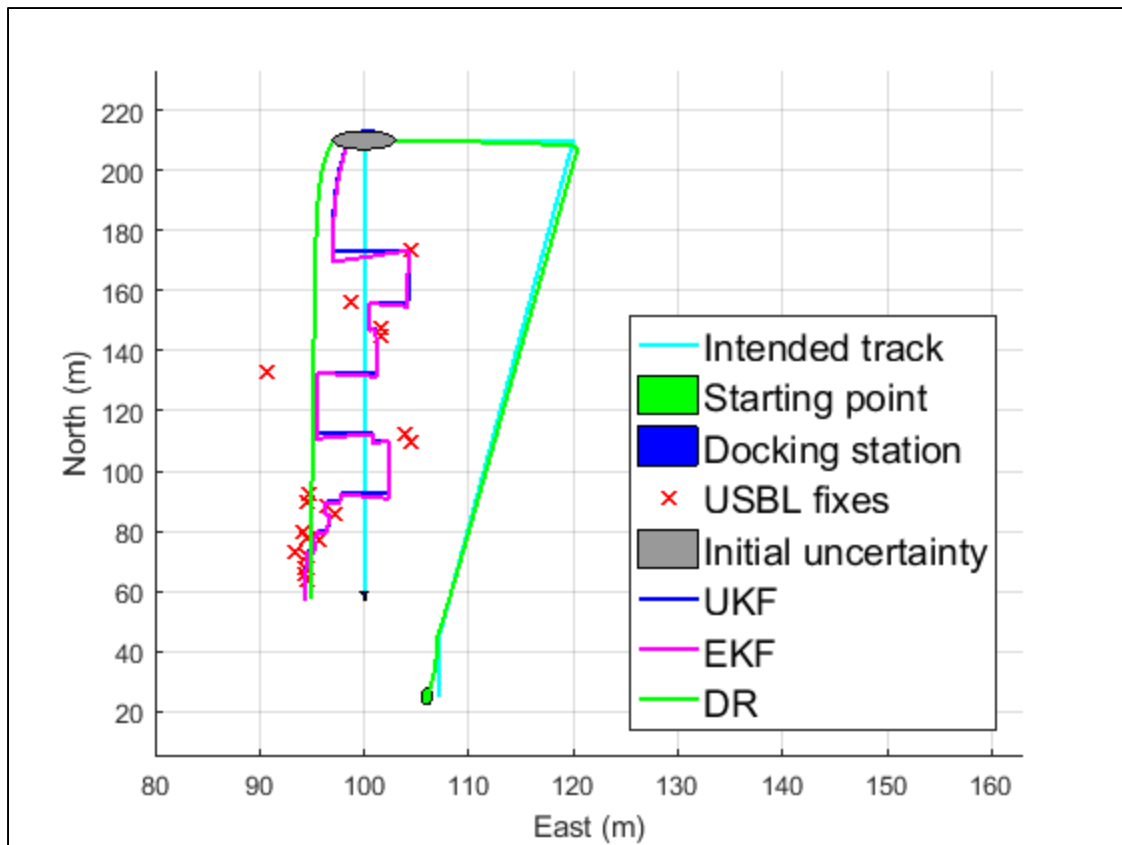
Figure 20. Run 7 with Lowest Update Rate and Poor Docking Results
