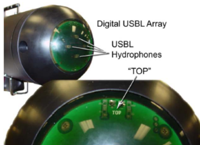
Figure 9. D-USBL Array in Its Nose Cap with Four-Channel Planar Hydrophone Array. Source: [3].
