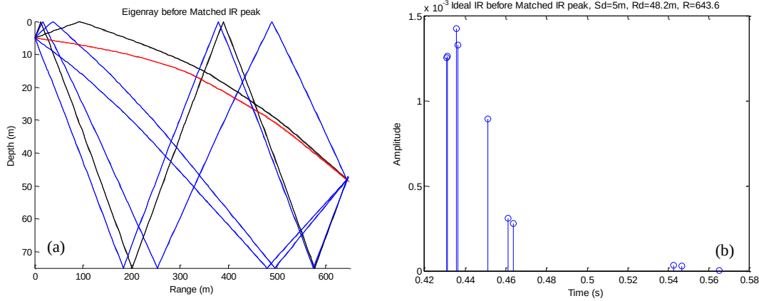
Figure 27. (a) Eigenrays and (b) Ideal IR before Matched Peak IR Processing. Data from Example 3
