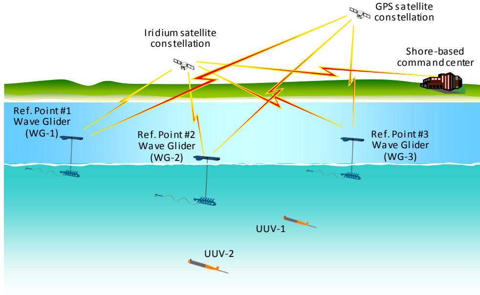
Figure 34. Simulation Scenario
