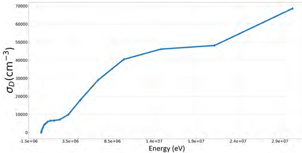
Figure 5.13. Displacement Cross Section for N-14 vs. Incoming Neutron Energy
