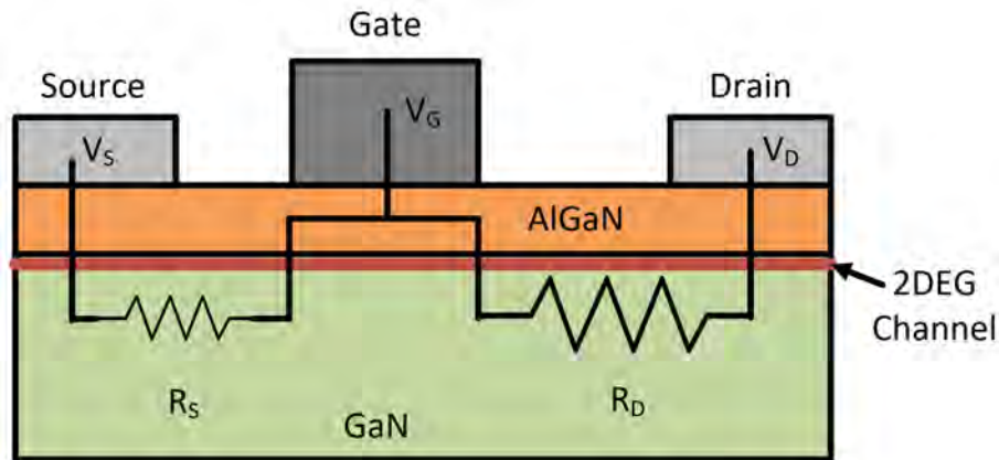
Figure 2.3. Illustration of the Cross Section of a GaN/AlGaN HEMT
