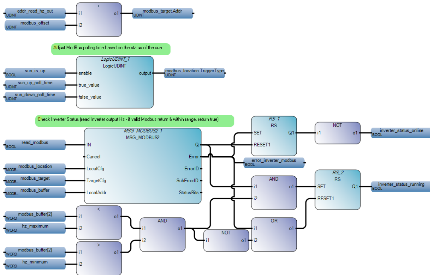
Figure 29. CheckInverterStatus FBD
