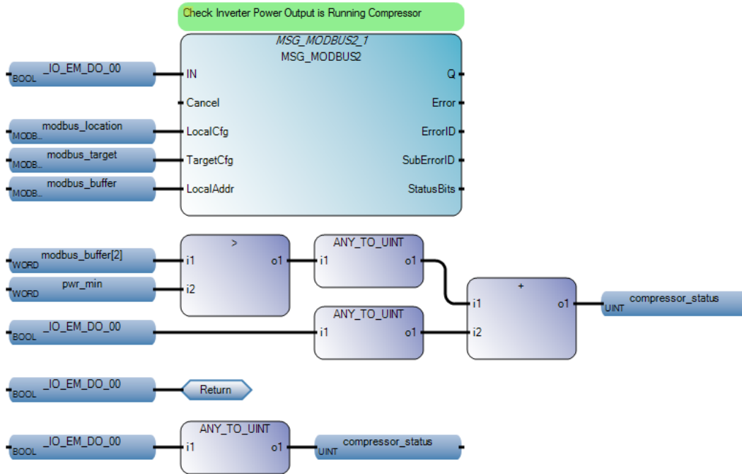
Figure 35. UpdateCompressorState FBD
