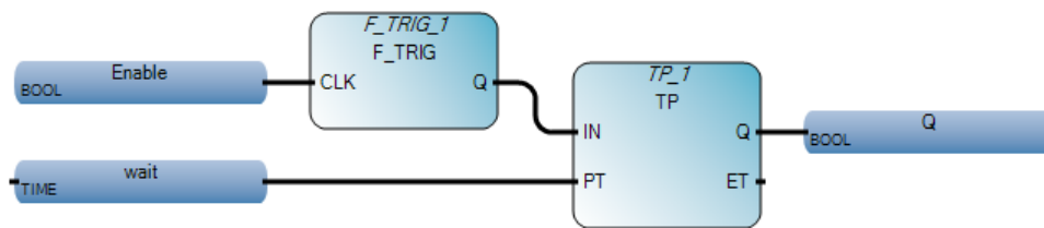
Figure 36. F_OneSecTrigger FBD
