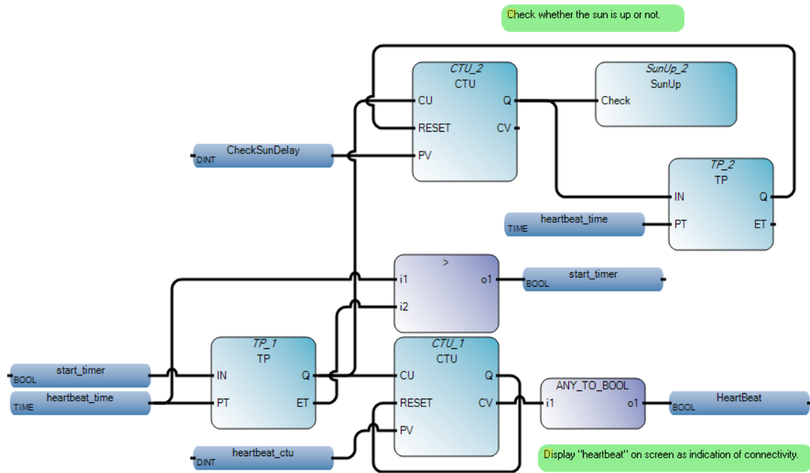
Figure 26. Heartbeat Program Function Block Diagram
