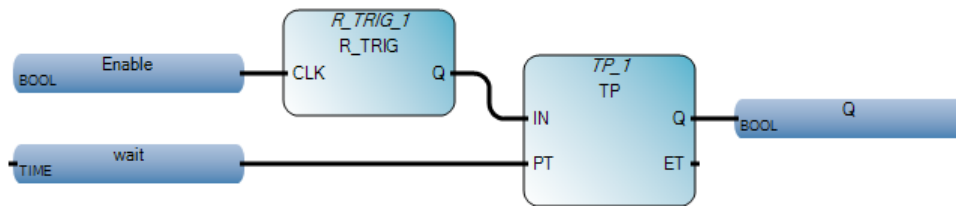
Figure 37. R_OneSecTrigger FBD
