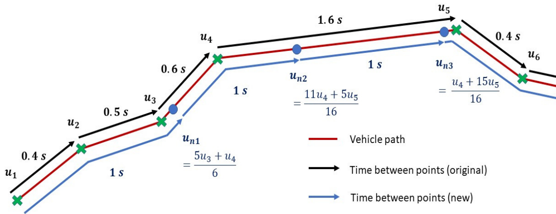
Figure 42. Creation of New Points at Discrete Time Intervals
