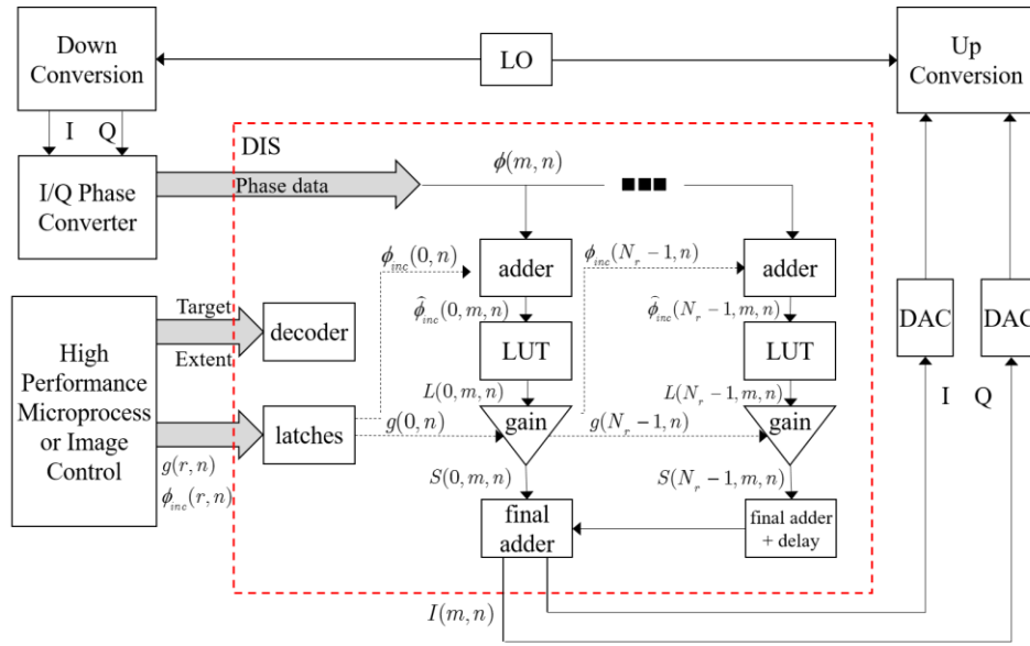
Figure 11. DIS Block Diagram. Adapted from [1].
