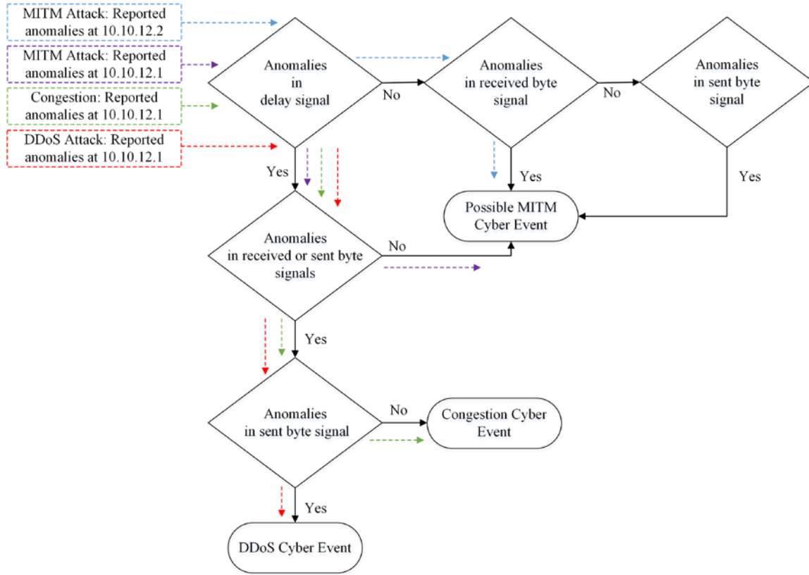
Figure 36. Cyber Event Classification
