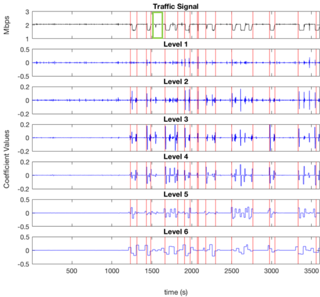
Figure 34. Congestion Detection in Received Byte Signal at Host 10.10.12.1
