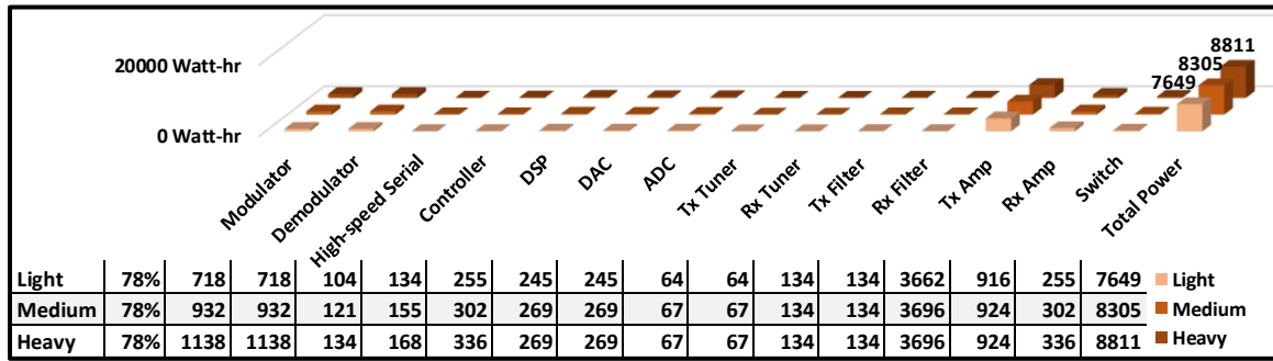
Figure 17. S-RTac EWC Architecture Component Power Simulation
