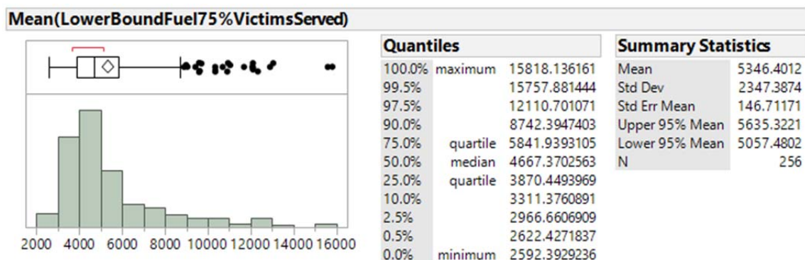
Figure 38. Histogram for Mean Lower Bound Fuel Consumed to Resupply 75% of Victim Clusters (Second Phase Experiment).
