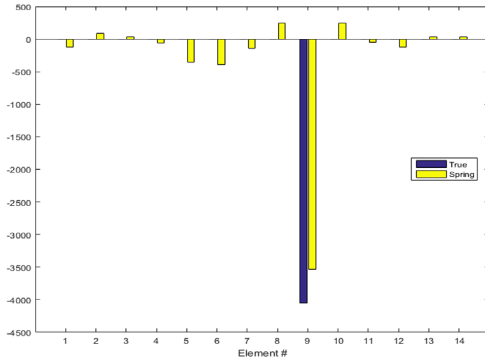
Figure 128. Two Spring Error Identification at Element 9
