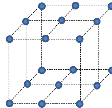
General Factorial 3 \times 3 \times 2 design
