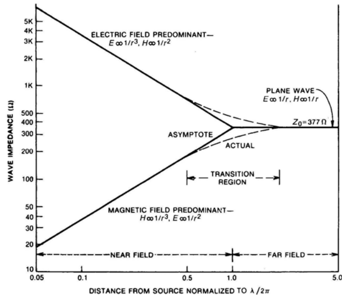
Figure 14. Wave Impedance Relationship to the Distance from the Source.
