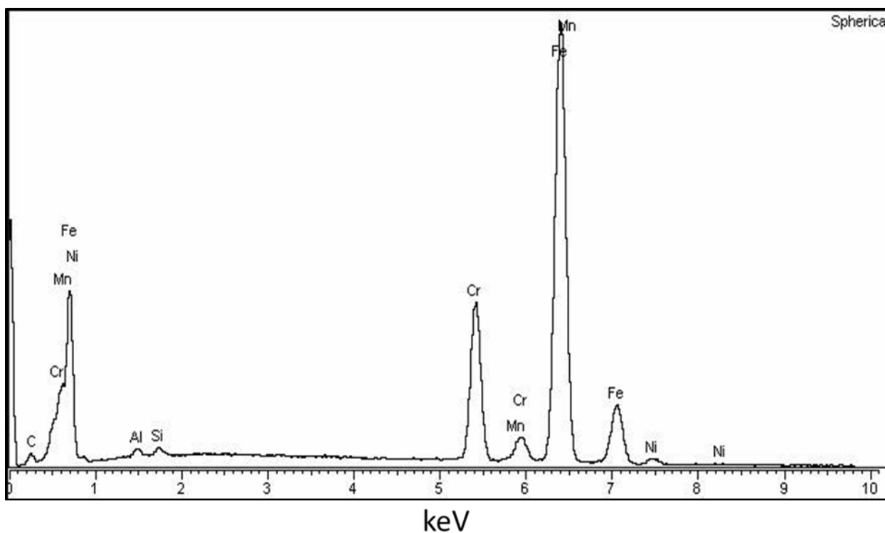
Figure 7 – EDS spectrum of SS 431 powder.
