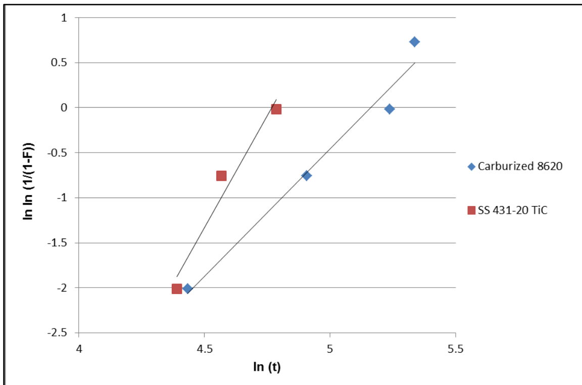
Figure 63 – Weibull plot of rolling contact fatigue life time for the carburized 8620 steel and laser deposited SS 431/20 TiC.
