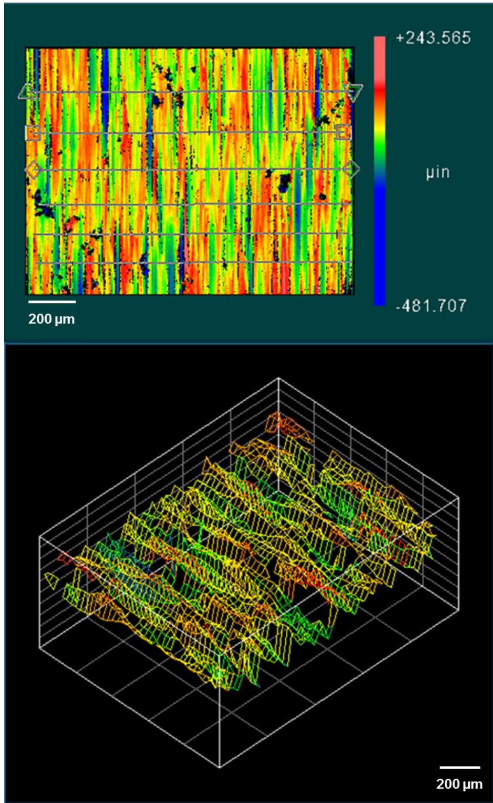
Figure 82 – Optical profilometry results of SS 431/20 TiC deposited onto Inconel 718 ® shaft.
