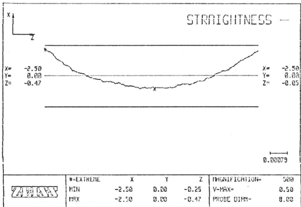
Figure 65 – Tribology analysis results of carburized 8620 steel roller before RCF testing.
