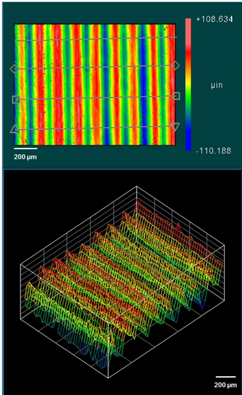
Figure 79 – Optical profilometry results of Inconel 718 ® shaft.
