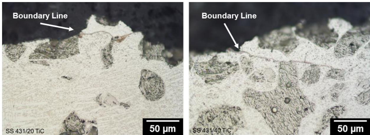
Figure 50 – Boundary lines which appeared in each deposition sample.
