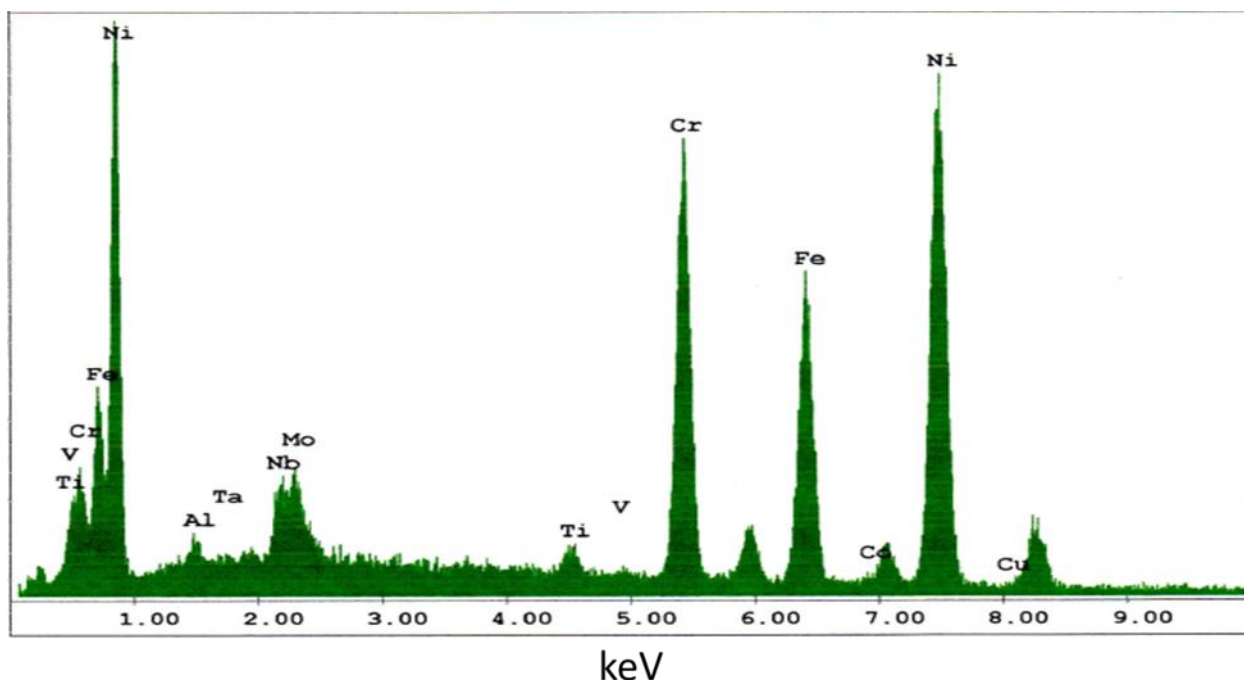
Figure 15 – EDS spectrum of Inconel 718 ® powder.
