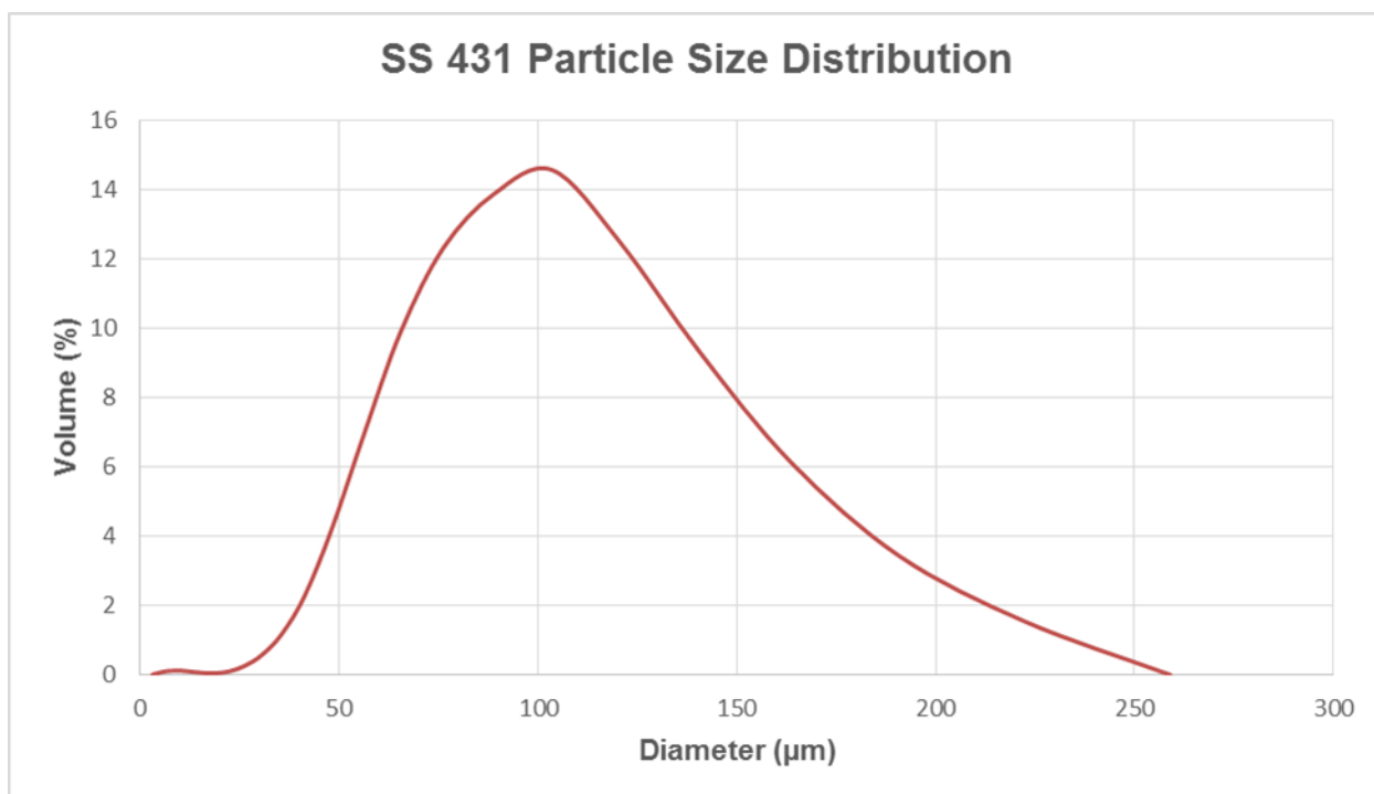
Figure 6 – Particle size distribution of SS 431 powder.
