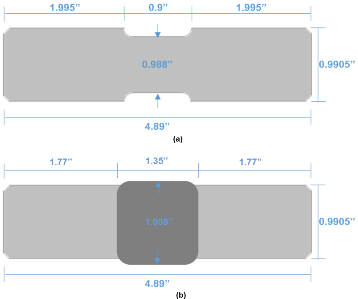
Figure 27 – Schematics of the specimen produced for RCF testing (a) initial machined specimen. (b) Specimen after with laser deposition materials over the center of carburized 8620 steel bar (Units are inches).
