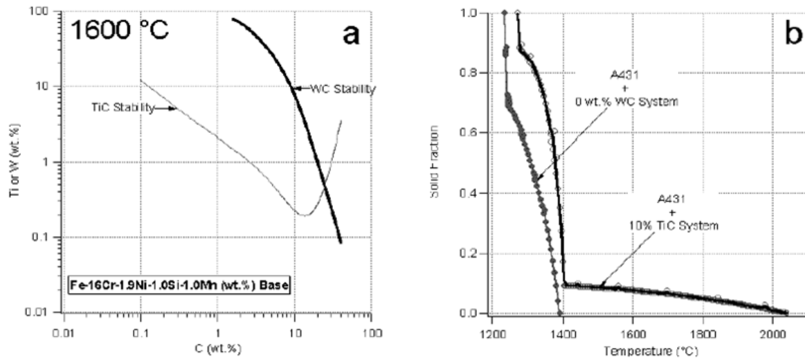
Figure 22 – Thermodynamic stability diagram (a) and solid volume fraction during cooling (b) for a system represented by titanium or tungsten with carbon in SS 431. [19]
