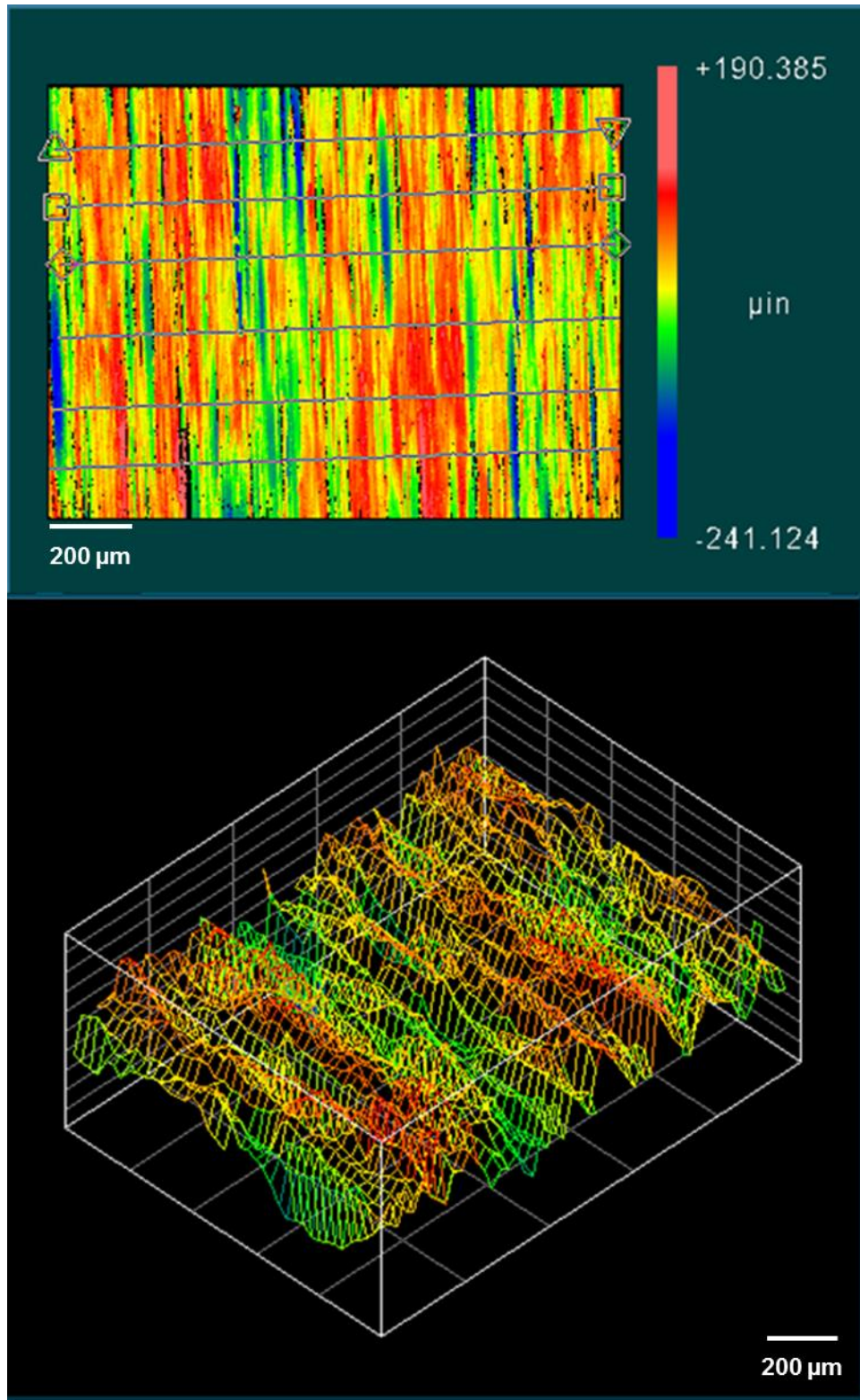
Figure 80 – Optical profilometry results of Inconel 718 ® deposited onto Inconel 718 ® shaft.
