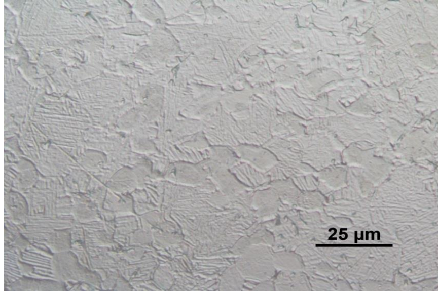
Figure 37 – Micrograph of unaffected Ti-6Al-4V substrate cooler fan shaft.
