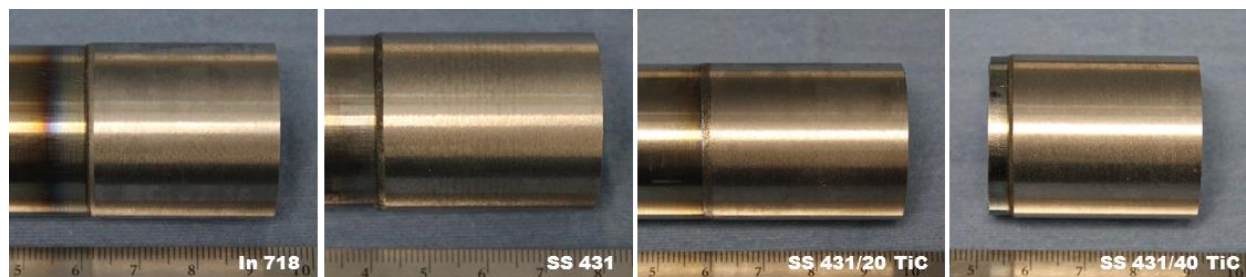
Figure 70 – Laser deposited materials on Inconel 718 ® power shaft after roller grind machining (scale in cm).
