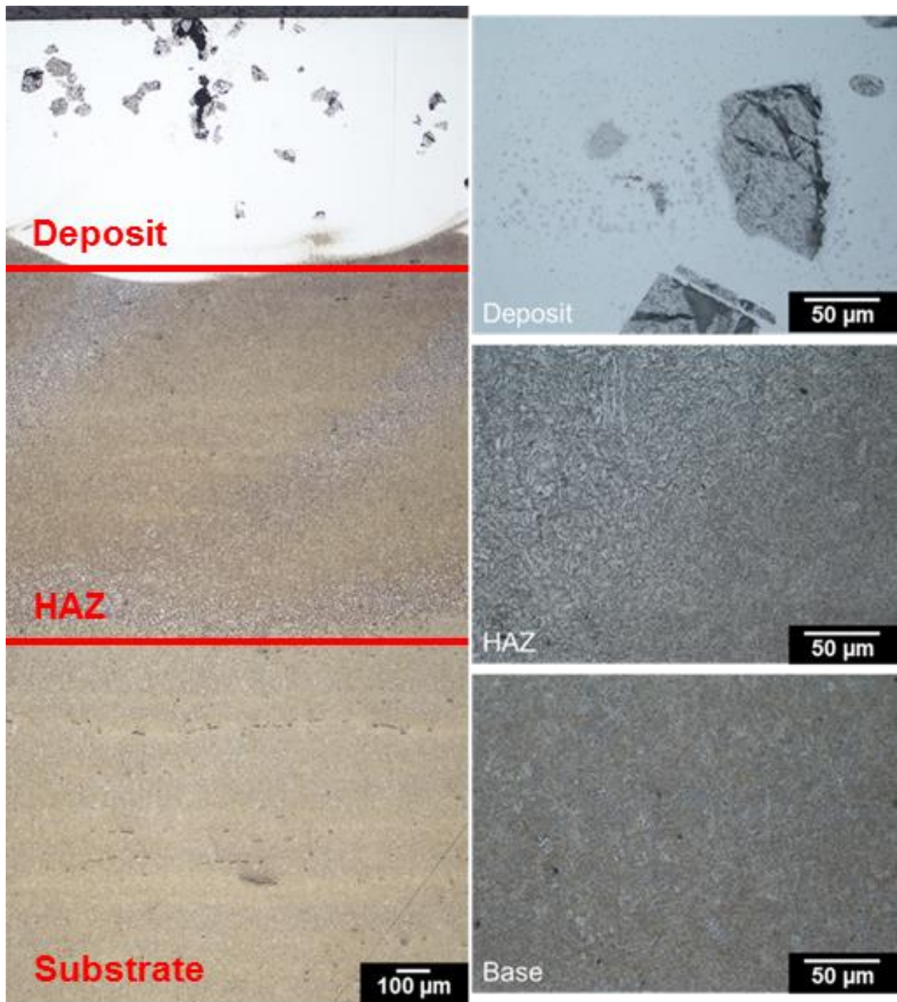
Figure 52 – Microstructures of RCF test specimen with laser deposited SS 431/20 wt% TiC representing transverse cross-section.
