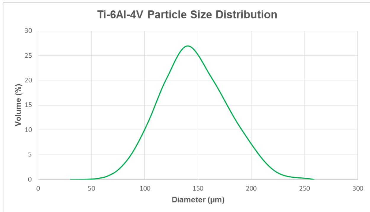
Figure 18 – Particle size distribution of Ti-6Al-4V ELI grade powder.
