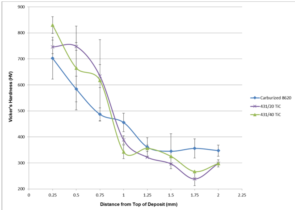
Figure 48 – Hardness profile with four different mixtures of SS 431 and TiC on carburized 8620 steel.
