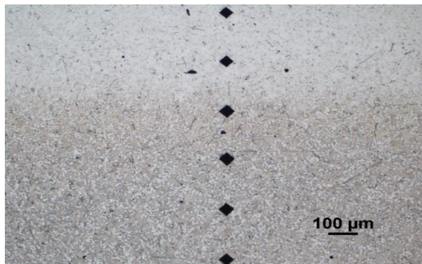
Figure 35 – Microhardness Measurement cooler fan shaft.
