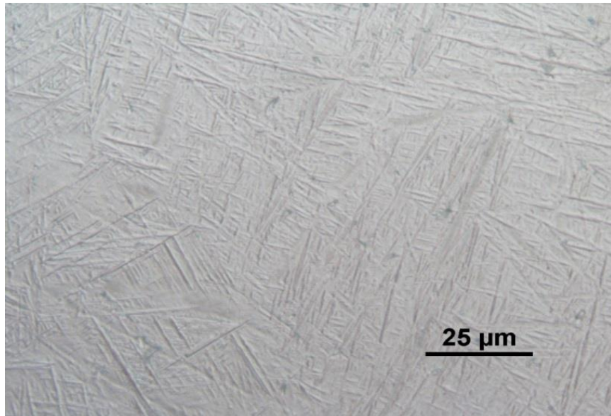
Figure 38 – Micrograph of Ti-6Al-4V deposit cooler fan shaft.
