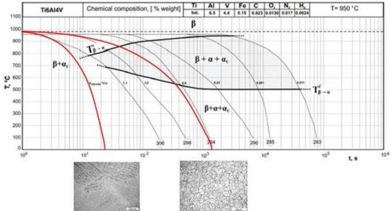
Figure 39 – Analysis of deposition and substrate based on Ti-6Al-4V CCT Diagram.
