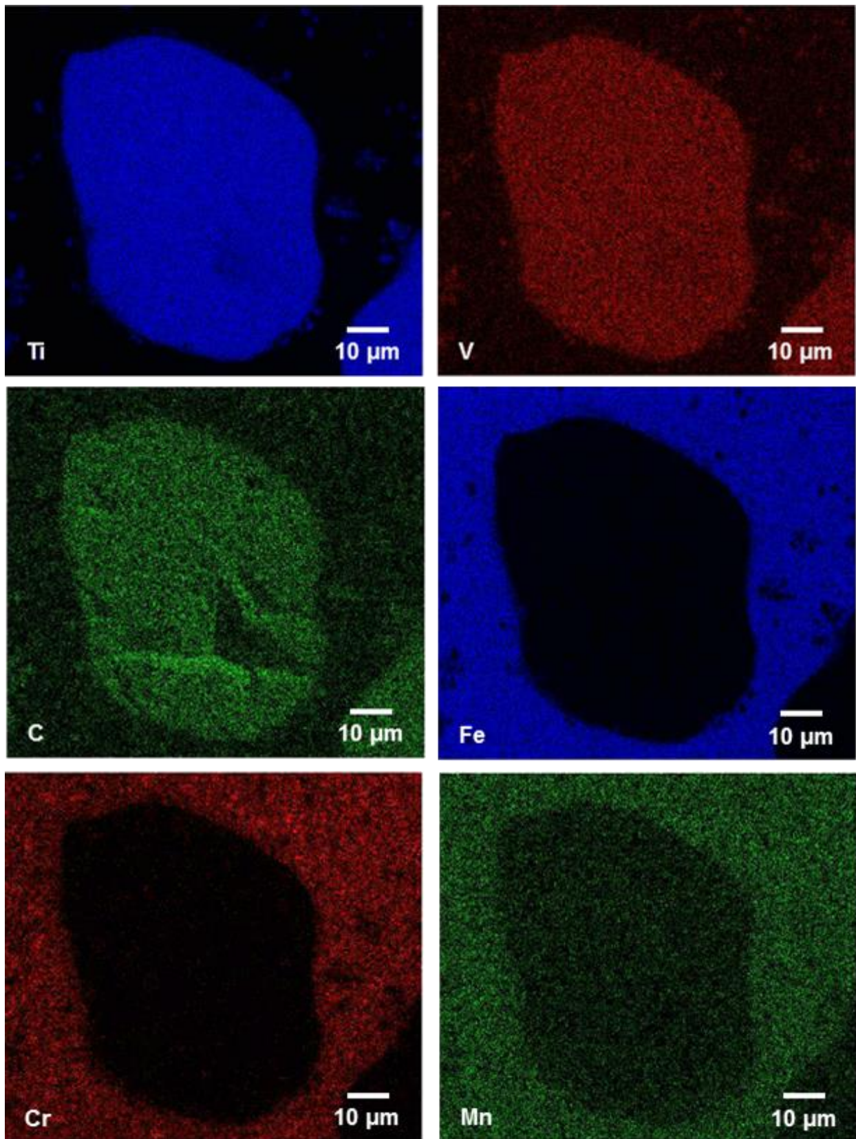
Figure 55 – Images generated by EDS mapping analyzer. Each image shows the respected element located from Figure 52.
