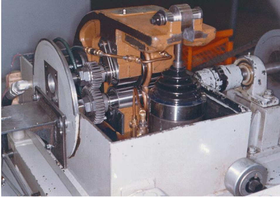
Figure 59 – Photograph of the rolling contact fatigue test at the Drivetrain Technology Center of the Applied Research Laboratory.
