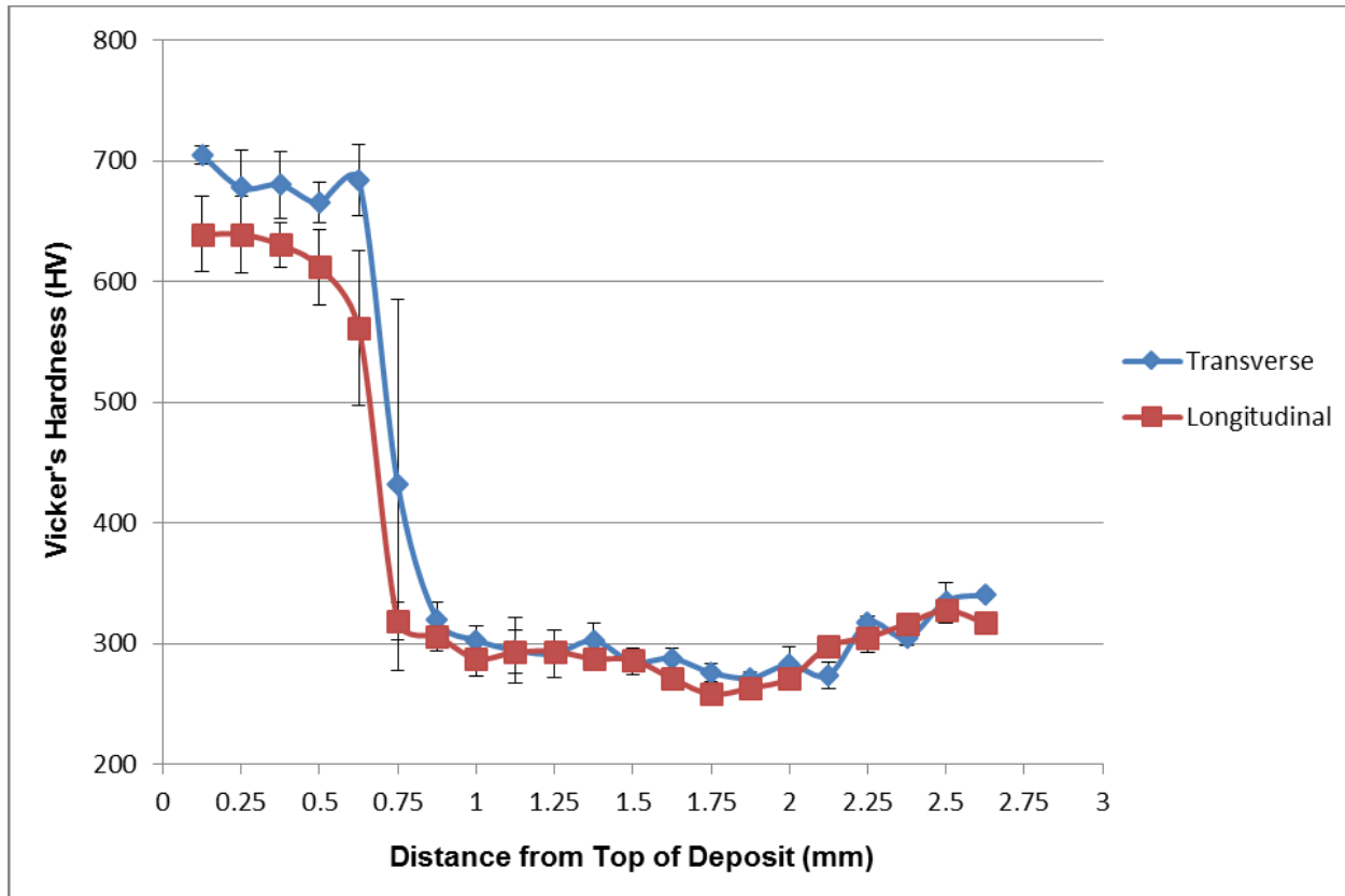
Figure 51 – Hardness profile of SS 431/20 TiC laser deposited on 8620 carburized steel of transverse and longitudinal cross-sections.
