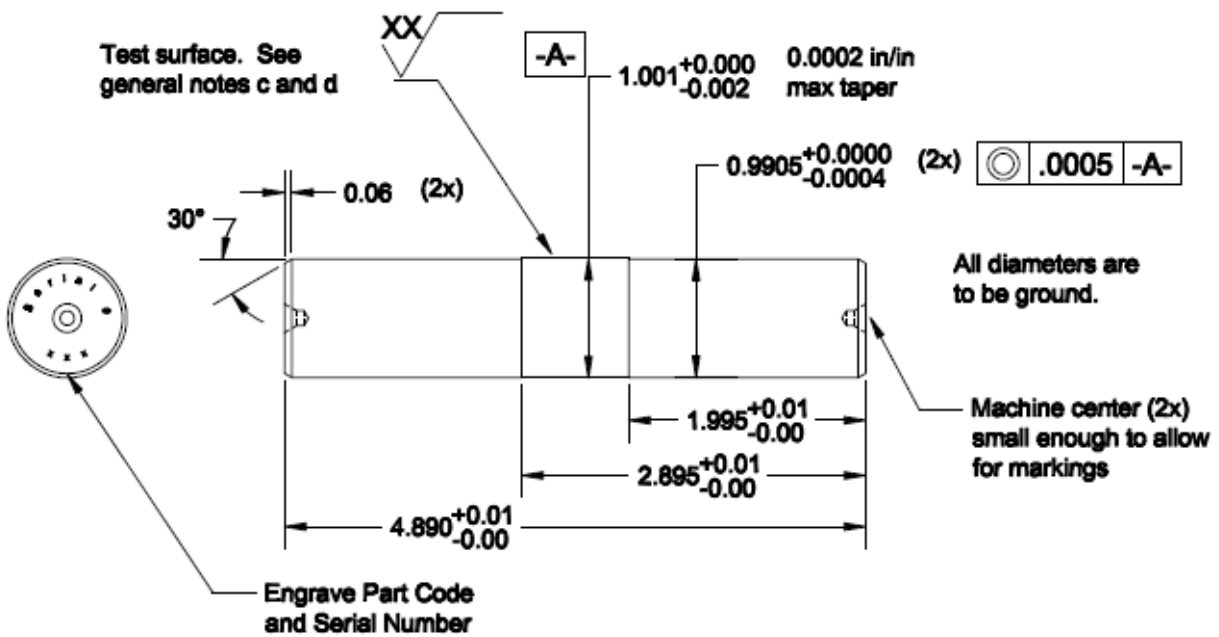
Figure 29 – The final dimension of the RCF test specimen.
