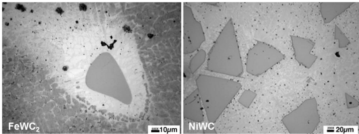
Figure 21 – Dissolution of WC particle in iron (left) and nickel (right). [19]
