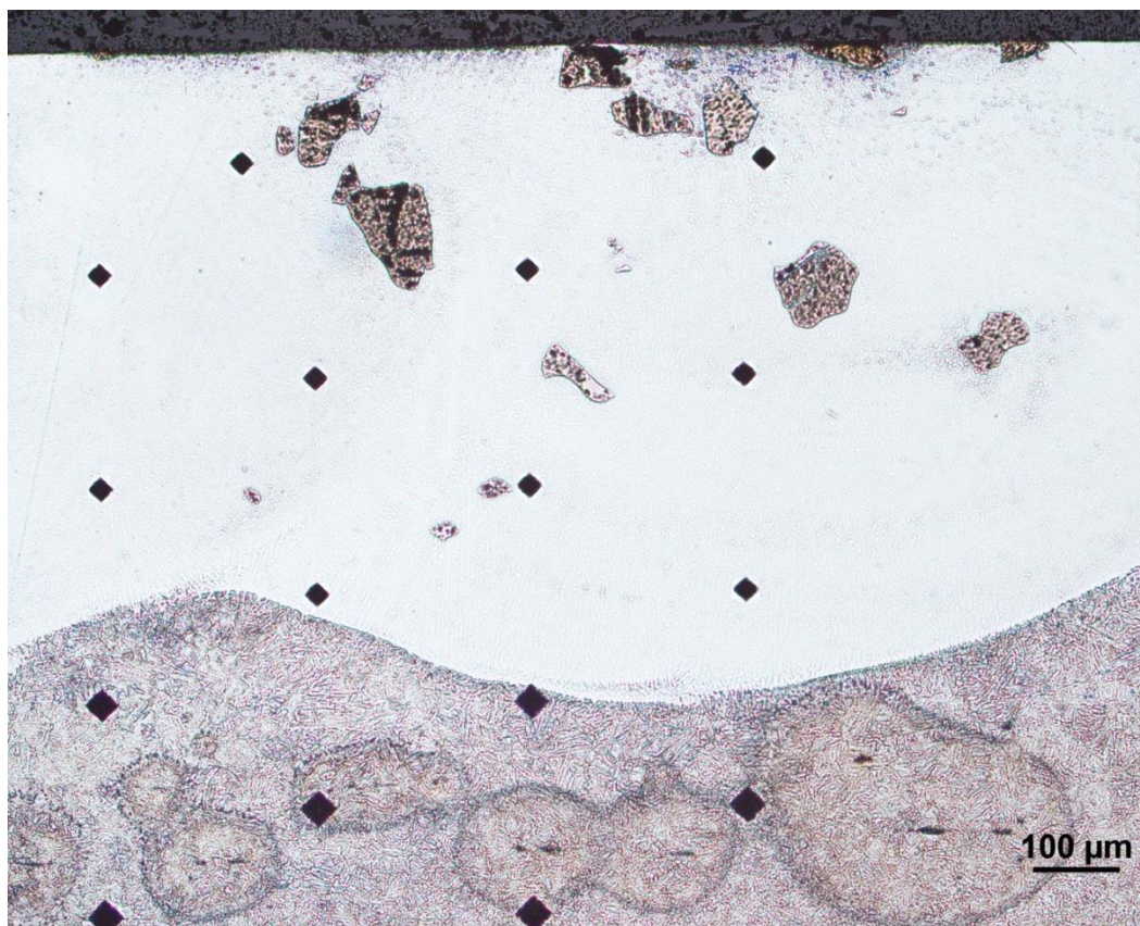
Figure 26 – Demonstrating the staggered procedure for measuring micro hardness.
