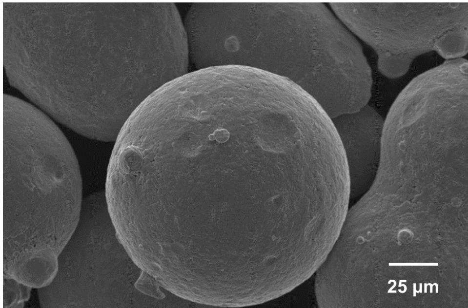
Figure 13 – SEM image of dense spherical Inconel 718 ® particle of powder obtained from Sulzer Metco.
