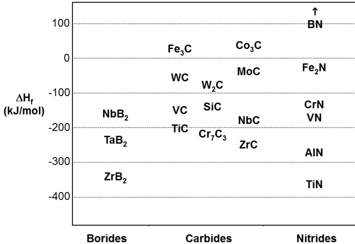
Figure 20 – Enthalpy of formation, \Delta H_f , of various hard phases. [19]
