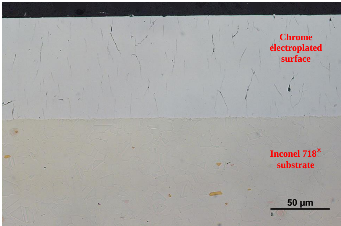
Figure 71 – Microstructural images of Inconel 718 ® shaft with chrome electroplated surface.
