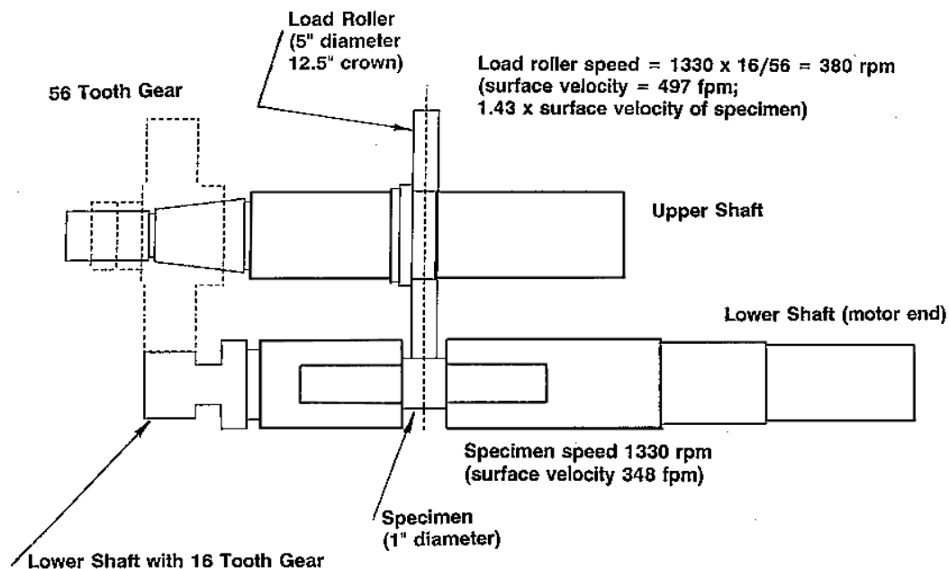
Figure 58 – Schematic of the rolling contact fatigue test. [21]
