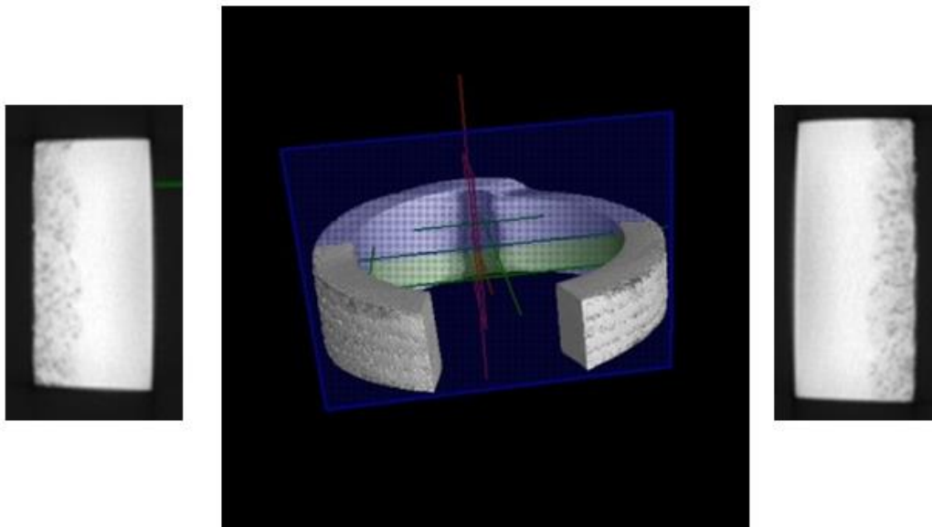
Figure 42 - Radiographic-based tomography of cooler fan shaft.
