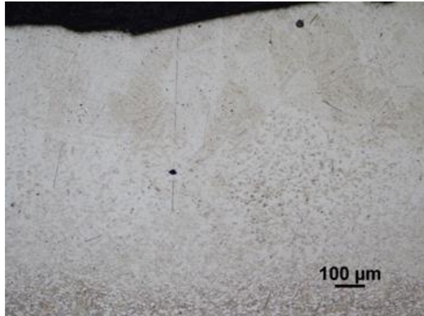
Figure 40 – Micrographic analysis for Microporosity of Ti-6Al-4V deposit.
