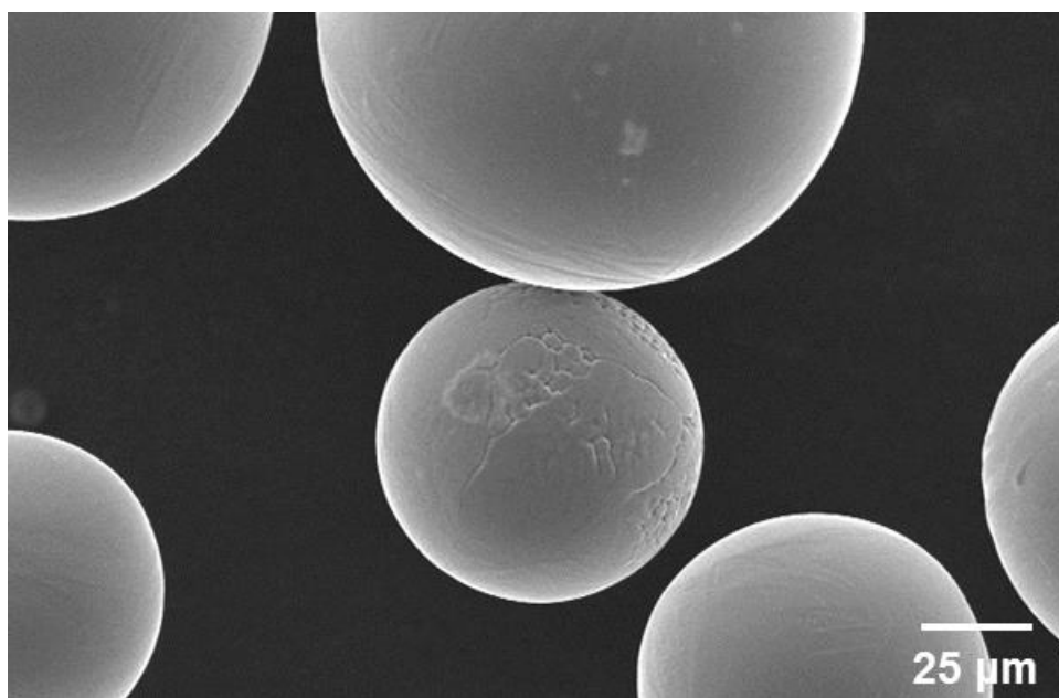
Figure 17 – SEM image of dense spherical Ti-6Al-4V ELI grade particle of powder obtained from Phelly Materials.
