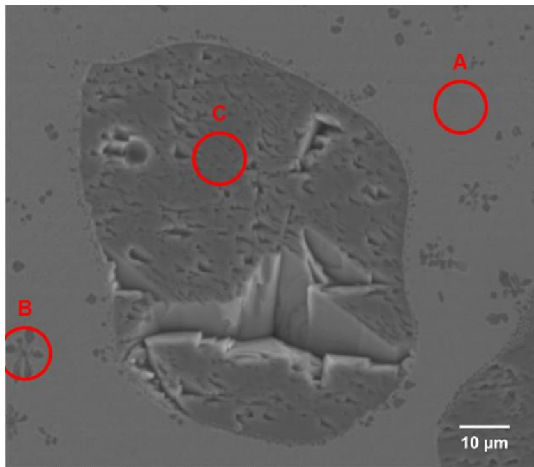
Figure 54 – SEM image of SS 431/20 TiC laser deposited material. Red circles indicate the area characterized by EDS analysis.
