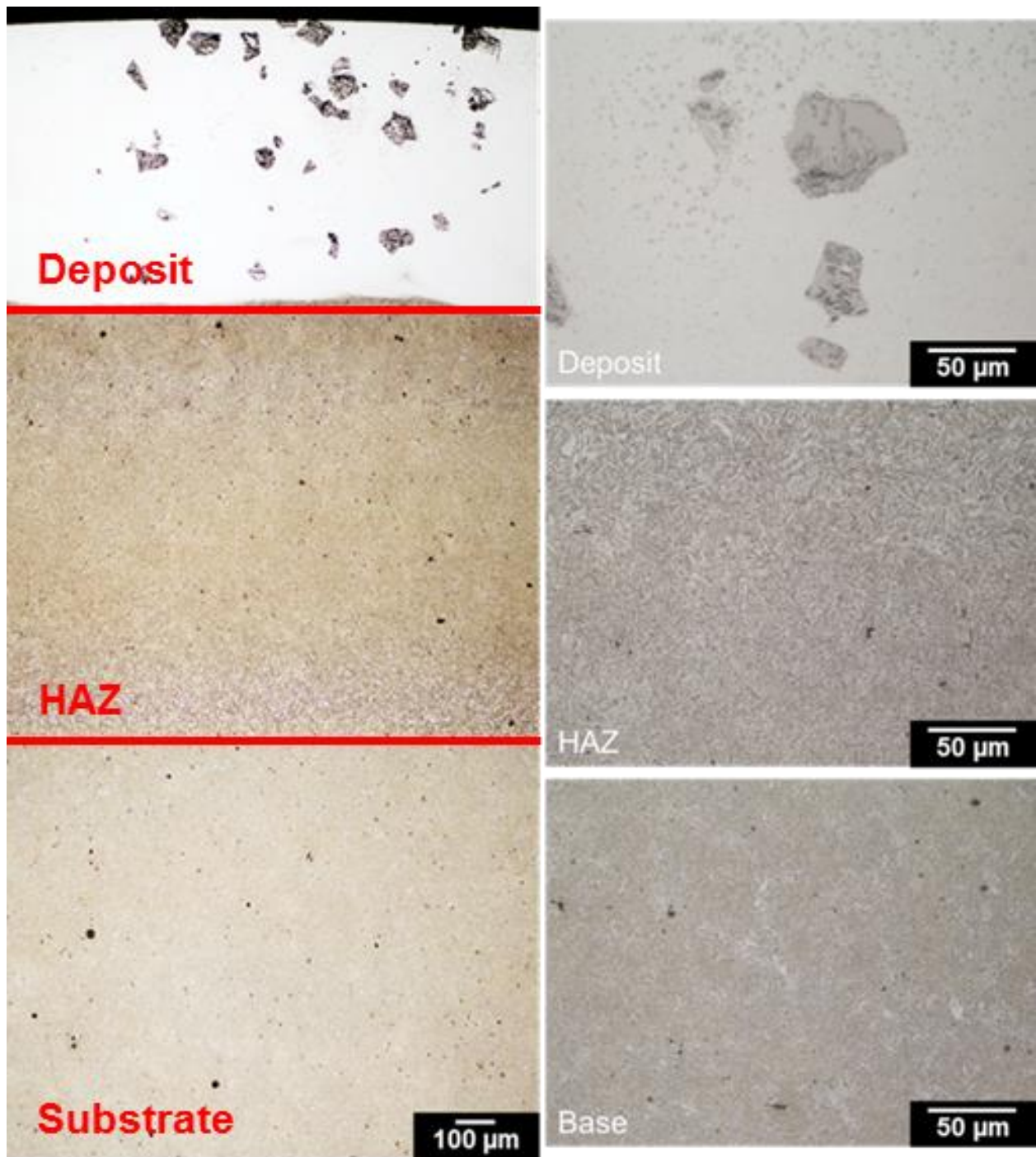
Figure 53 – Microstructures of RCF test specimen with laser deposited SS 431/20 wt% TiC representing longitudinal cross-section.
