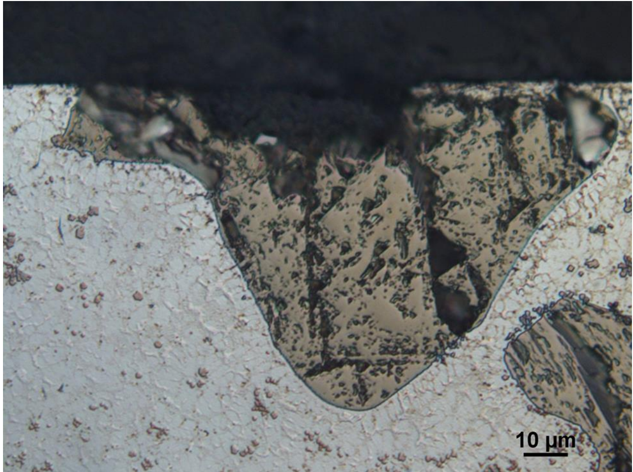
Figure 77 – Microstructural image showing the voids on the surface of RCF specimen.
