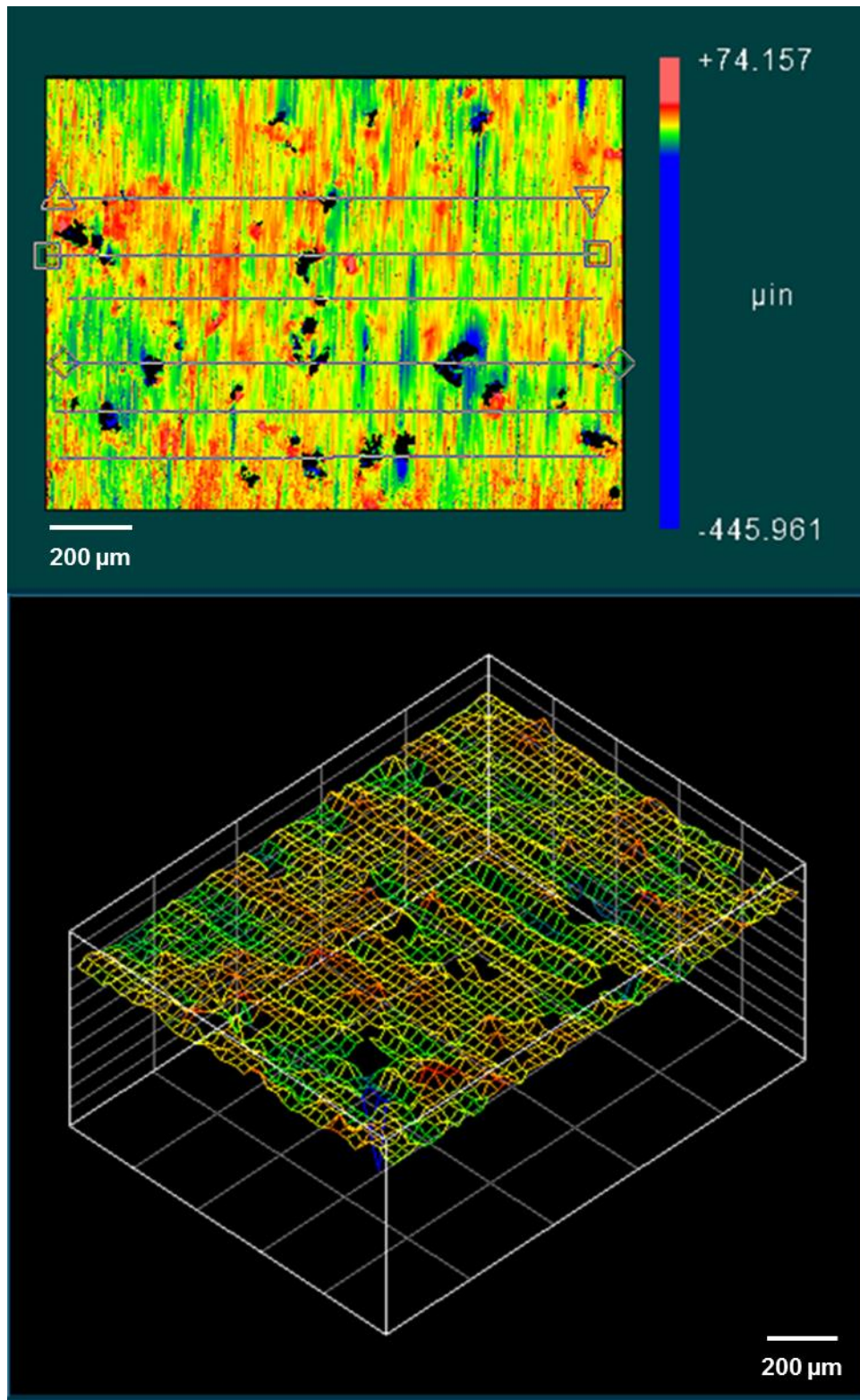
Figure 76 – Optical profilometry of the SS 431/20 TiC RCF test specimen, at the surface with defects.
