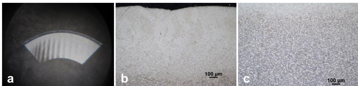
Figure 36 – (a) Macrograph longitudinal section cooling fan shaft. (b) Micrograph deposit and interface cooling fan shaft. (c) Micrograph interface, HAZ, and substrate.
