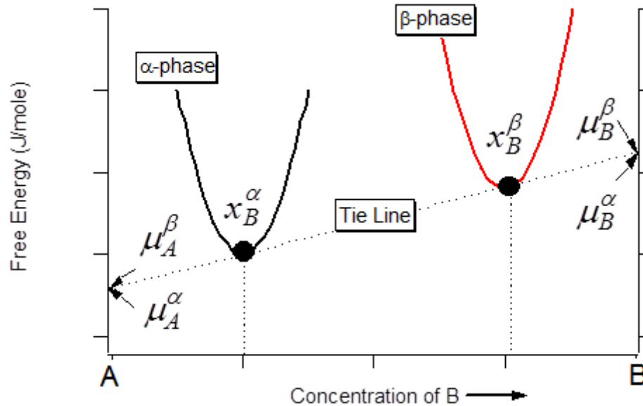
Figure 24 – Two-phase molar Gibbs energy diagram. [19]
