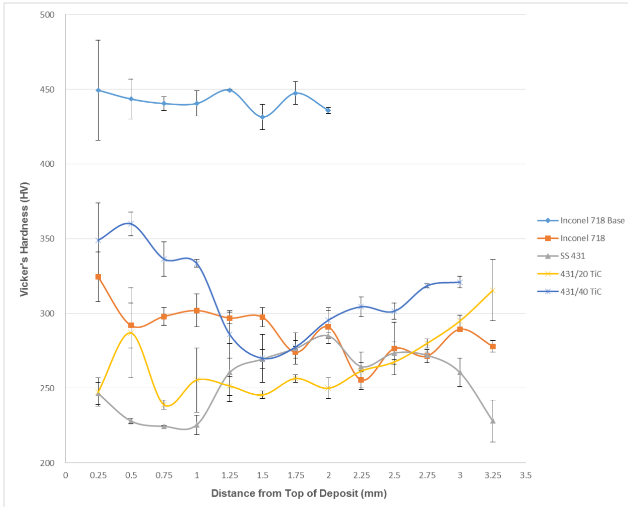
Figure 73 – Hardness of Inconel 718 ® shaft with deposited materials.
