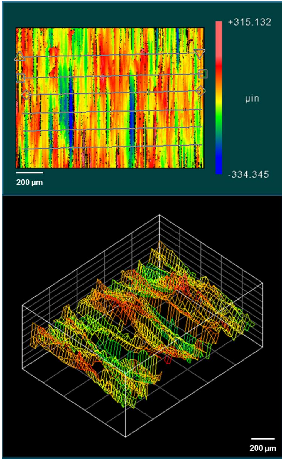
Figure 81 – Optical profilometry results of SS 431 deposited onto Inconel 718 ® shaft.
