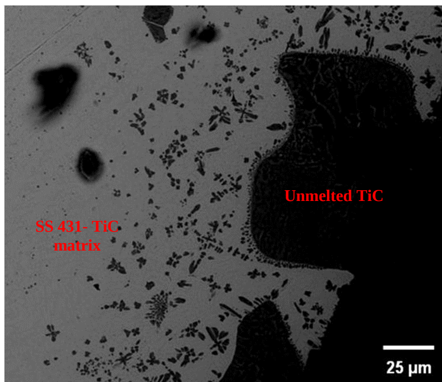
Figure 56 – SEM image showing TiC particles along with precipitates of TiC formed during cooling.
