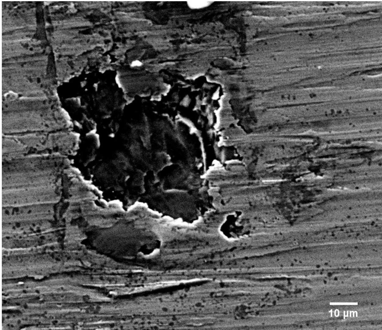
Figure 78 – SEM image shows the voids on the surface of RCF specimen.
