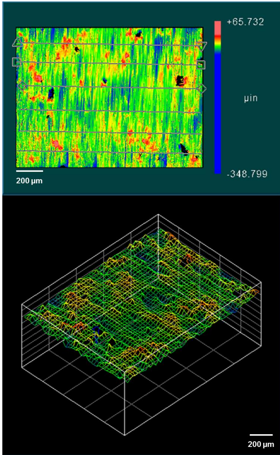
Figure 75 – Optical profilometry of the SS 431/20 TiC RCF test specimen, at the surface without defects.
