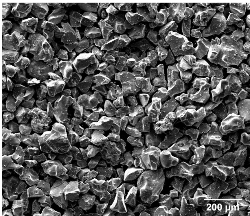
Figure 8 – SEM image of TiC particles of powder obtained from AEE Corporation.
