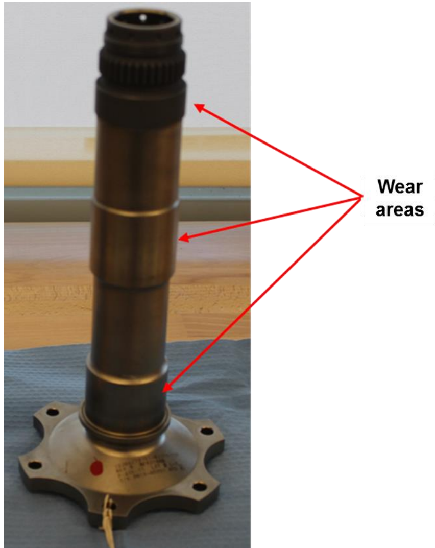
Figure 34 – Cooling fan shaft faults with bearing journal wear.
