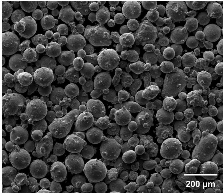
Figure 4 – SEM image of SS 431 particles of powder obtained from Carpenter Technology.
