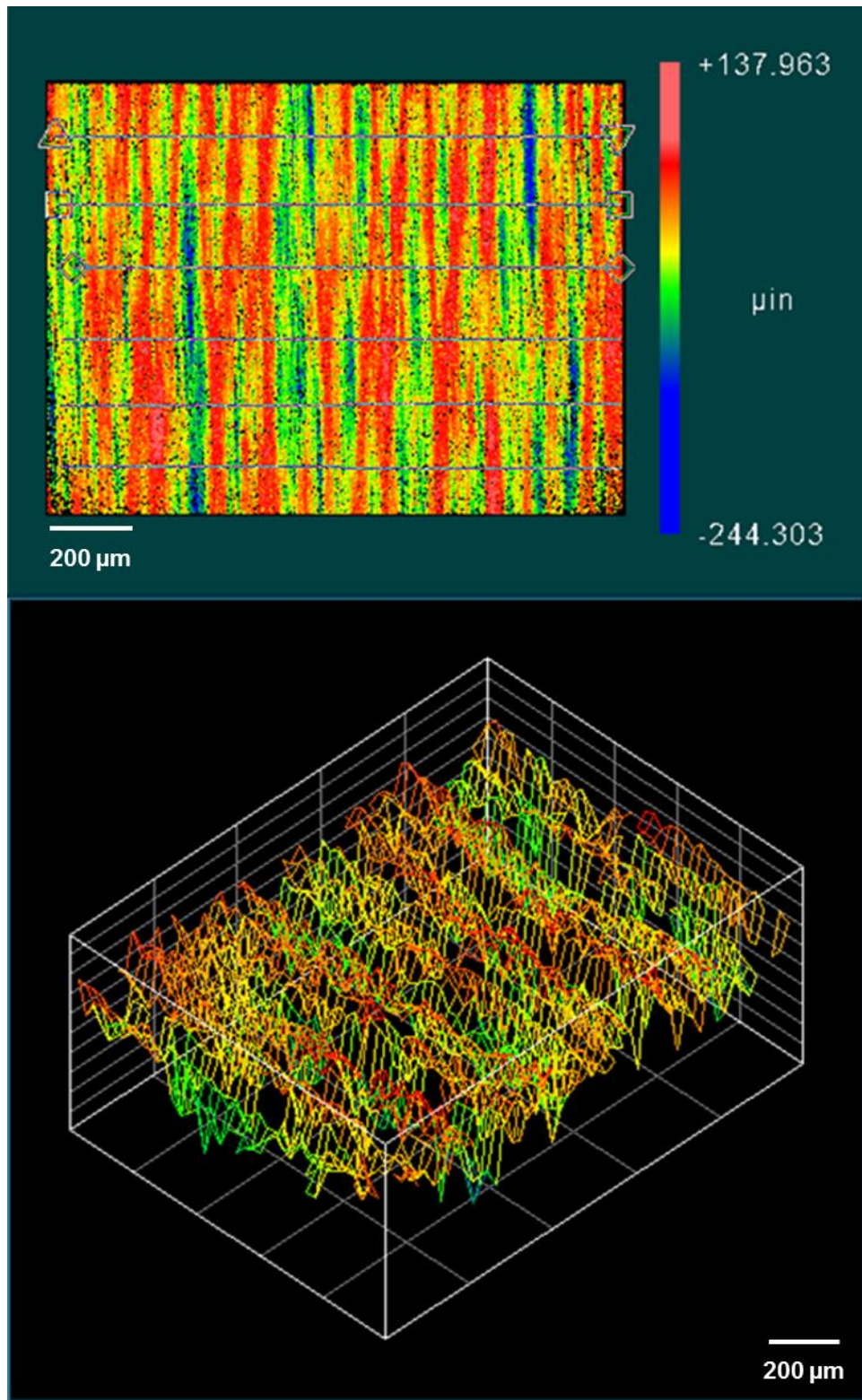
Figure 74 – Optical profilometry of the baseline carburized 8620 steel specimen used in the RCF test.
