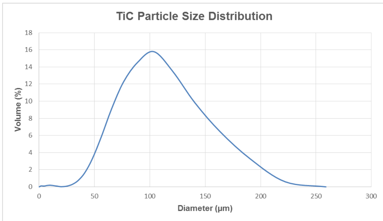
Figure 10 – Particle size distribution of TiC powder.
