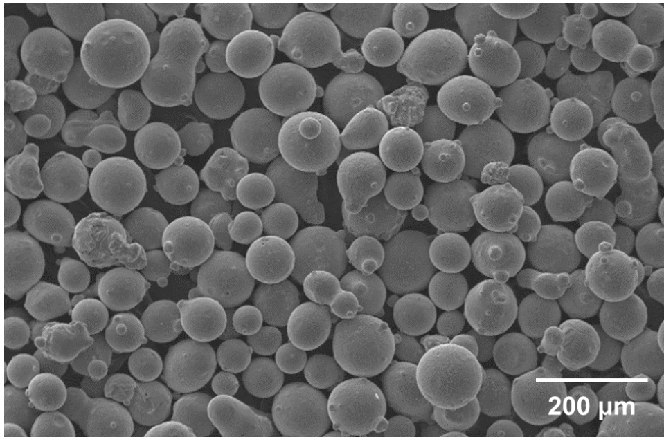
Figure 12 – SEM image of Inconel 718 ® spherical particles of powder obtained from Sulzer Metco.
