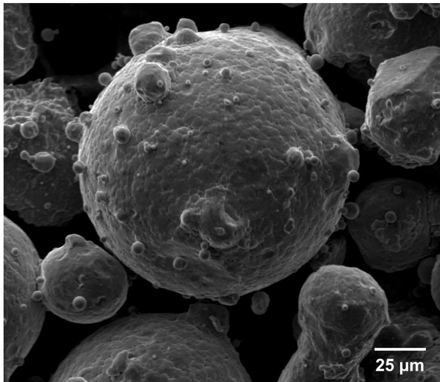
Figure 5 – SEM image of SS 431 particle with satellites around the dense spherical particle of powder obtained from Carpenter Technology.
