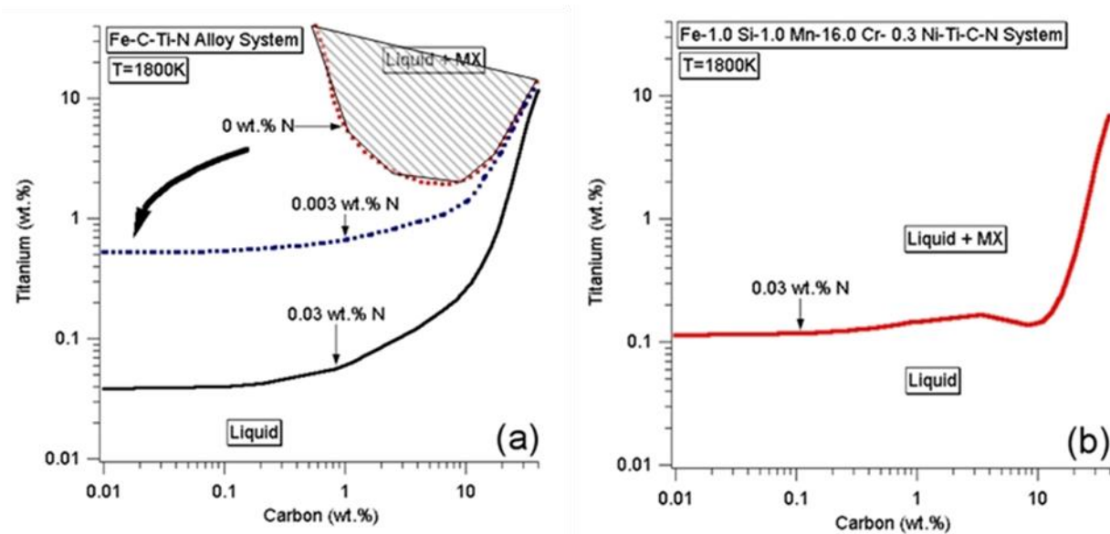
Figure 23 – Thermodynamic calculations of MX stability as a function of carbon and nitrogen for (a) a simple Fe-based and (b) complex Fe-base alloy. [19]
