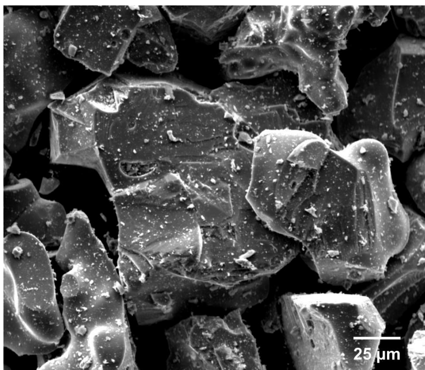
Figure 9 – SEM image of TiC particle with pores at the surface of powder obtained from AEE Corporation.
