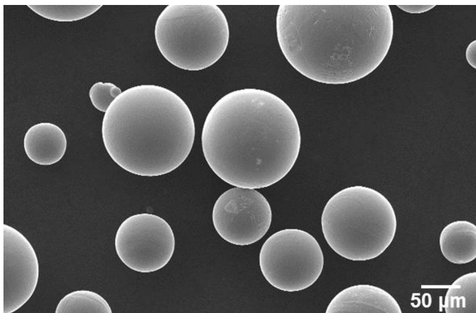
Figure 16 – SEM image of Ti-6Al-4V ELI grade spherical particles of powder obtained from Phelly Materials.
