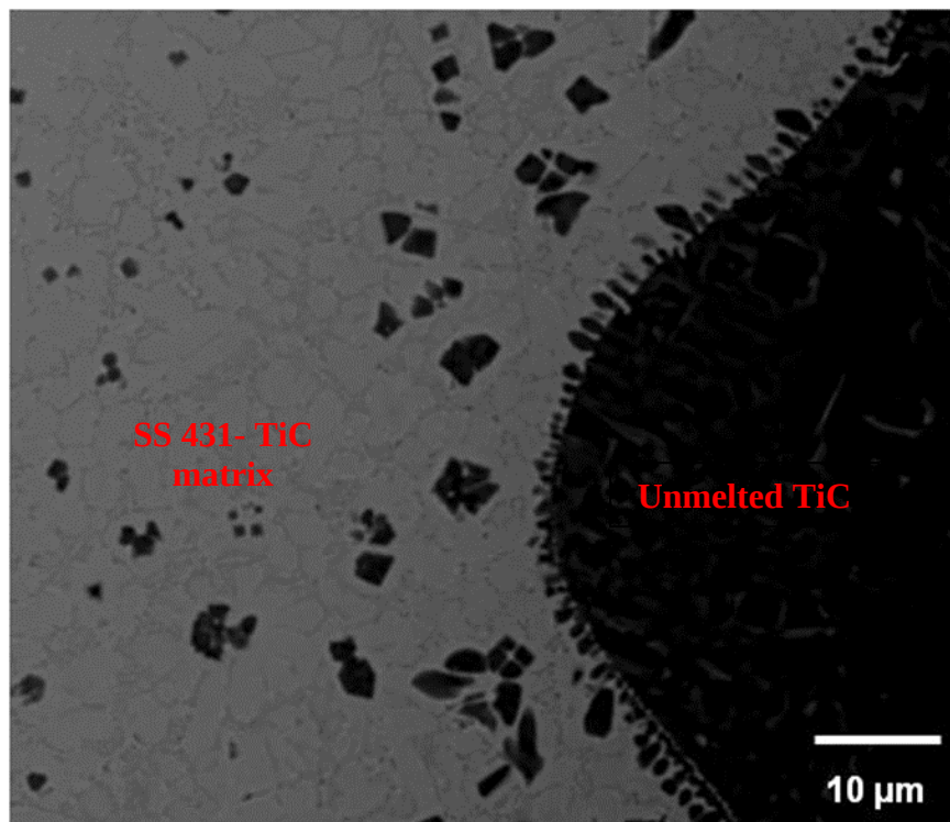
Figure 57 – SEM image showing TiC precipitation.
