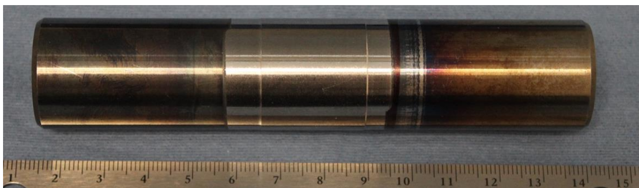
Figure 30 – The RCF test specimen with laser deposited SS 431/20 TiC (scale in cm).
