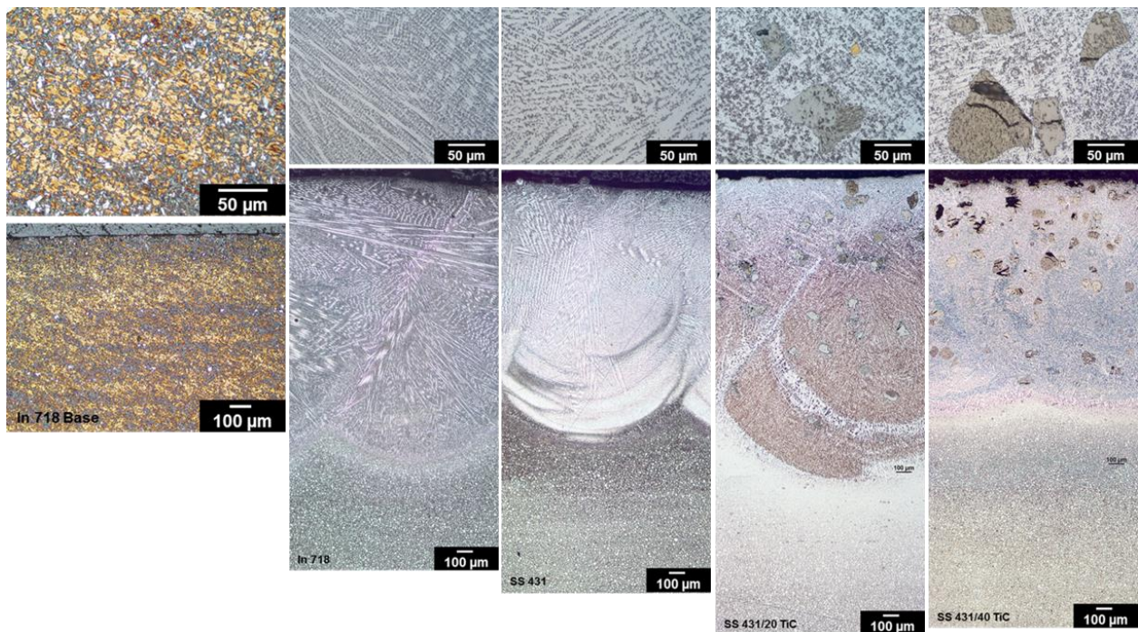
Figure 72 – Metallurgical analysis of the deposition material for the Inconel 718 ® power shaft.
