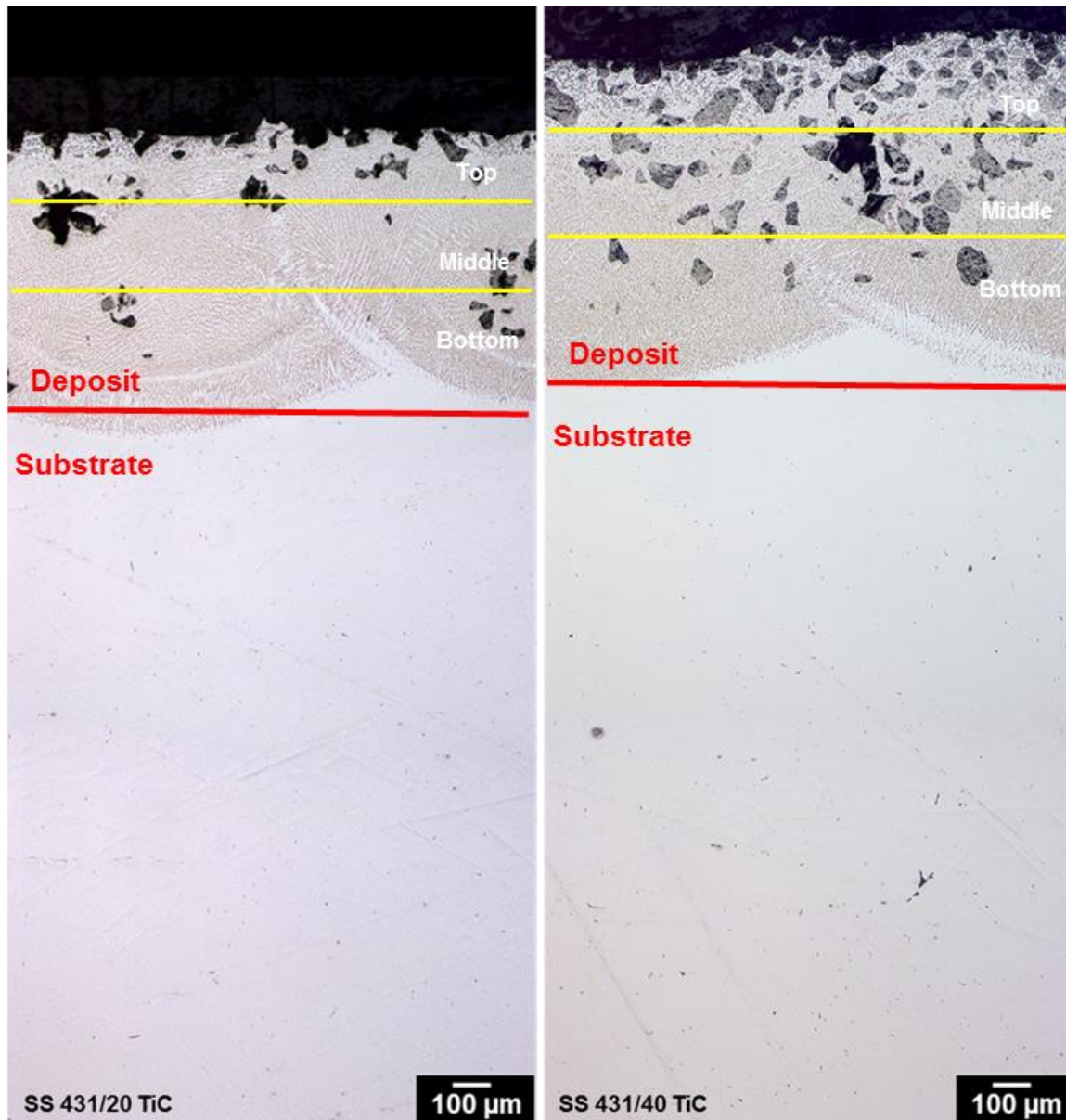
Figure 49 – Microstructure cross-section of each sample with respective deposit, HAZ, and 8620 base material.
