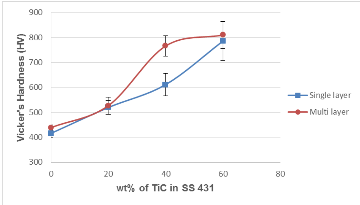
Figure 47 – Hardness of deposits produced using increasing amount of TiC blended in SS 431 powder that had been deposited on low carbon steel.
