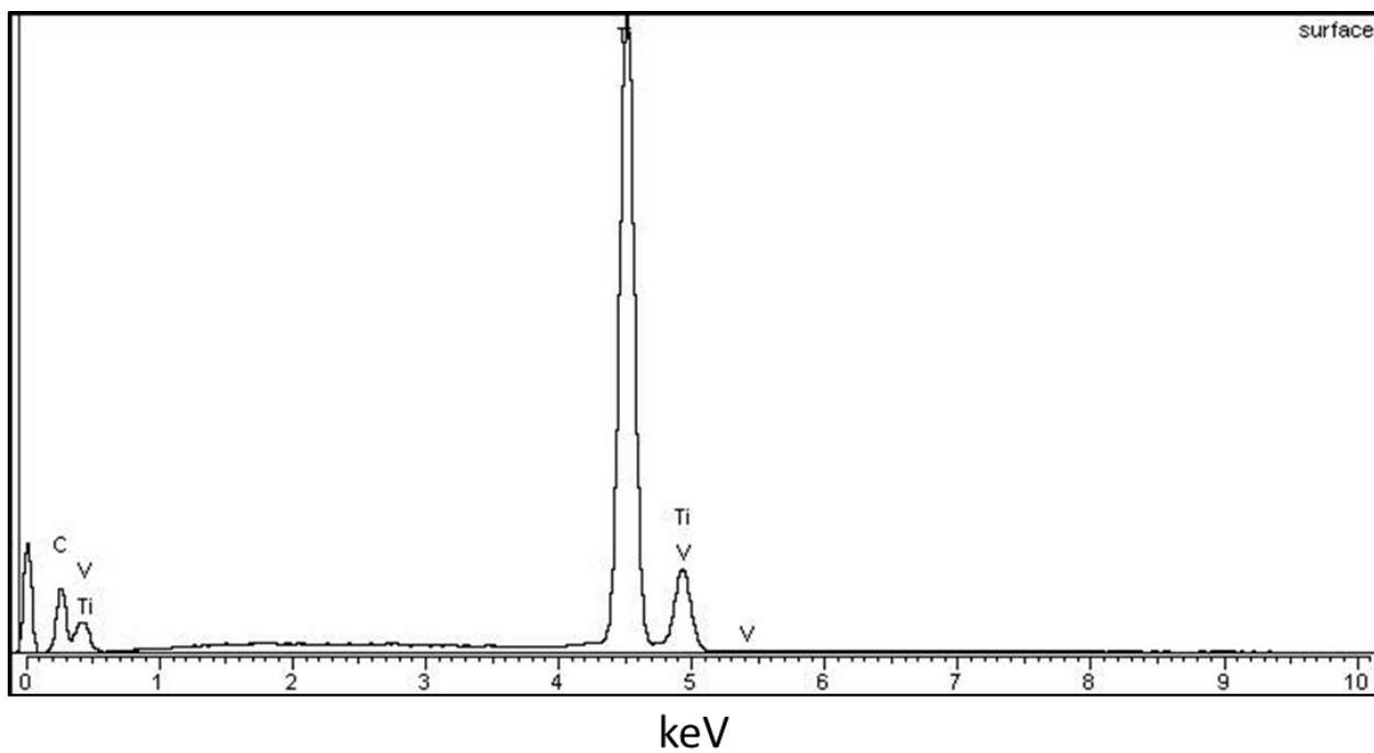
Figure 11 – EDS spectrum of TiC powder.
