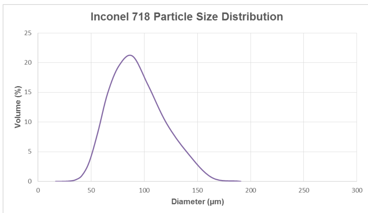
Figure 14 – Particle size distribution of Inconel 718 ® powder.
