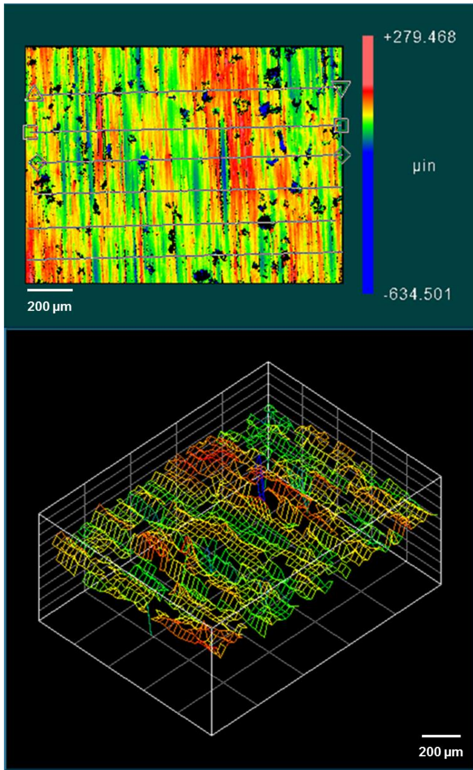
Figure 83 – Optical profilometry results of SS 431/40 TiC deposited onto Inconel 718 ® shaft.
