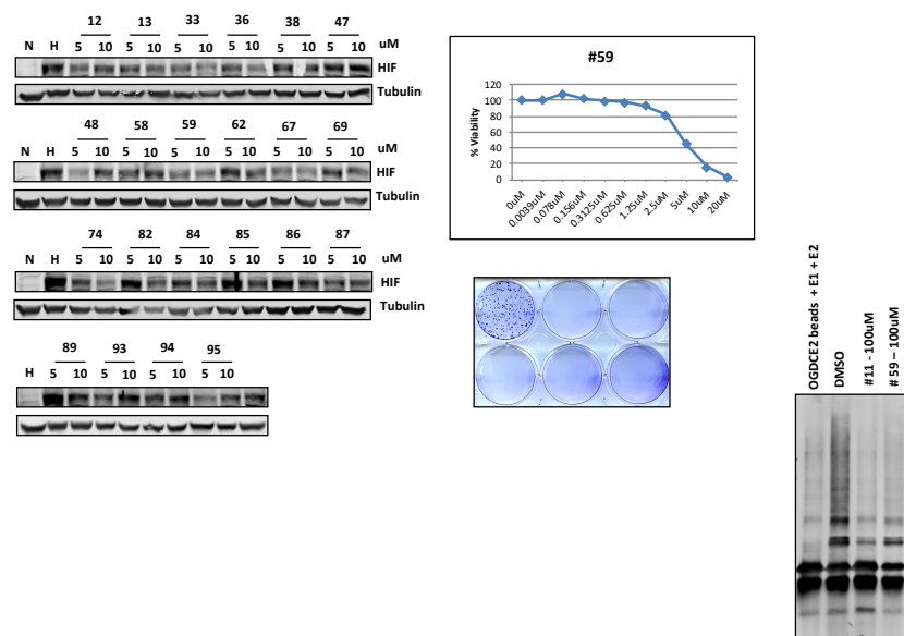
Figure 3. Effect of compound #59 on HIF1 \alpha , proliferation and ubiquitination. (A) Selected compounds (5 uM, 10 \mu M) from in silico -based screen were added to prostate tumor cells and cultured in 1% oxygen incubator overnight. HIF levels were examined by Western Blot analysis. (B) Compound #59, at the indicated concentrations, was added to prostate tumor cell line. Viability was assessed 72 h and colonies were stained 10 days after treatment. Upper panel depicts quantification of CFE shown on the lower panel (C) Compound #59 was incubated with Siah substrate OGDCE2 for half an hour followed by the addition of ubiquitination reagents (E1, E2, Ub). The mixtures were then incubated at 37°C for 45 min followed by Western Blot analysis.
