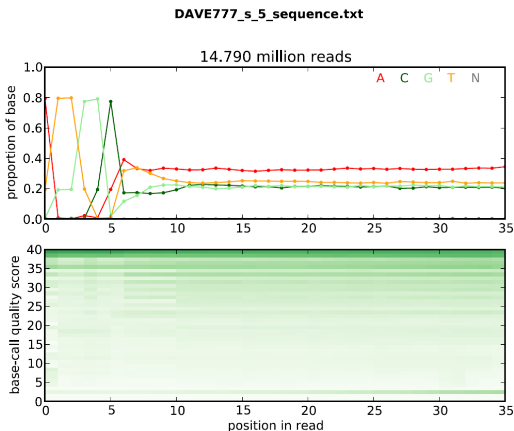
Figure 1: Base-level quality control reads as a function of position in read. The first seven
