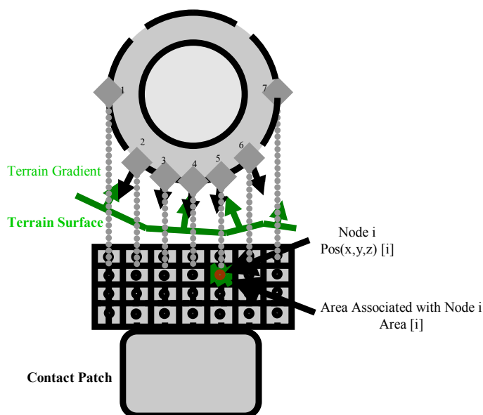
Figure E-13: Simplified Tire and Terrain Elements.
