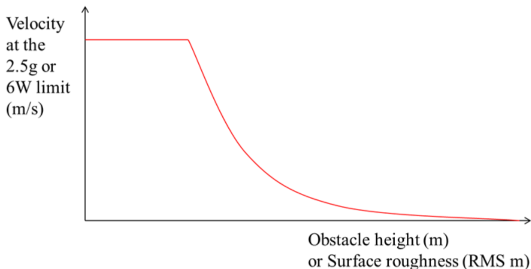
Figure 4-4: Generic VEHDYN Constraint Curve.
