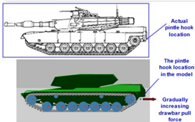
Figure E-15: Example of Tracked Vehicle Model Development.
