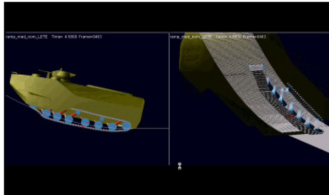
Figure E-16: Example Simulation Event – Gradeability on a Deformable Surface.
