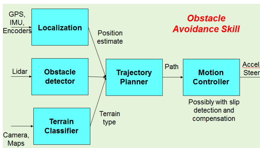
Figure 9-7: Illustration of the Hierarchical Nature of Skills Using the Obstacle Avoidance Skill Example.
