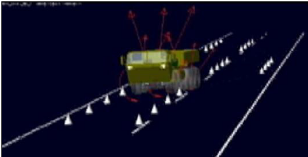
Figure F-4: LVSr-TD 10 x 10 Model During Double Lane Change Simulation.
