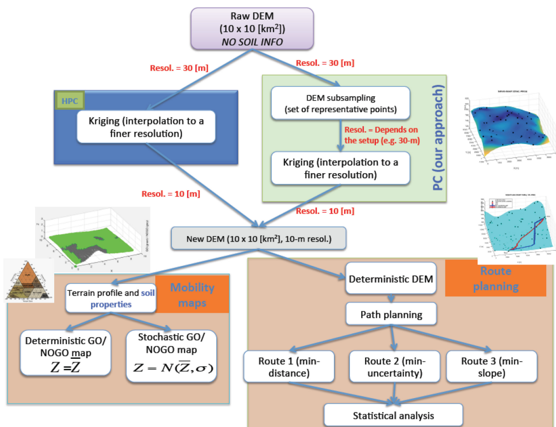
Figure 8-2: Schematic View of the Steps Carried out in the Proposed Architecture for Predicting the Mobility of a Ground Vehicle over a Large Region (> 5 x 5 [km²]).
