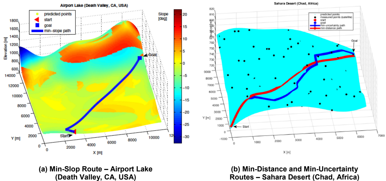
Figure 8-3: Routes Obtained Using the Global Path Planner. The mesh represents the terrain model considering nominal elevations (kriging estimations).
