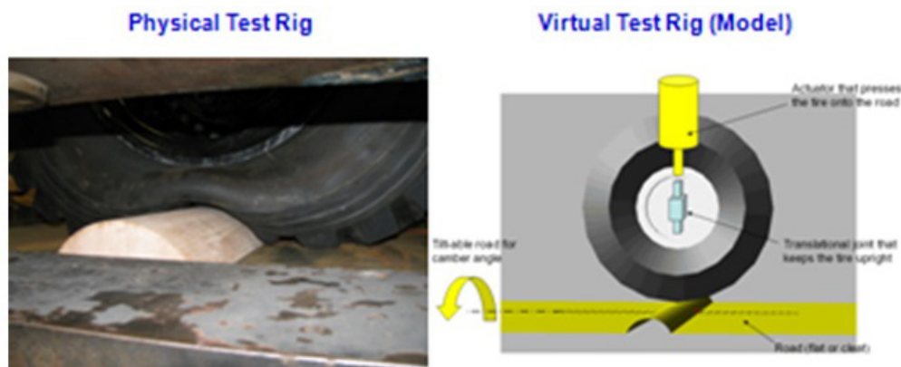
Figure E-12: Correlating Physical Testing with Simulation.
