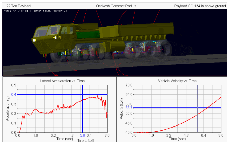
Figure E-4: Example of Synchronized Graphic and Time History Results.
