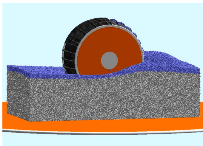
Figure E-14: Examples of Deformable Tire and Terrain Simulation.
