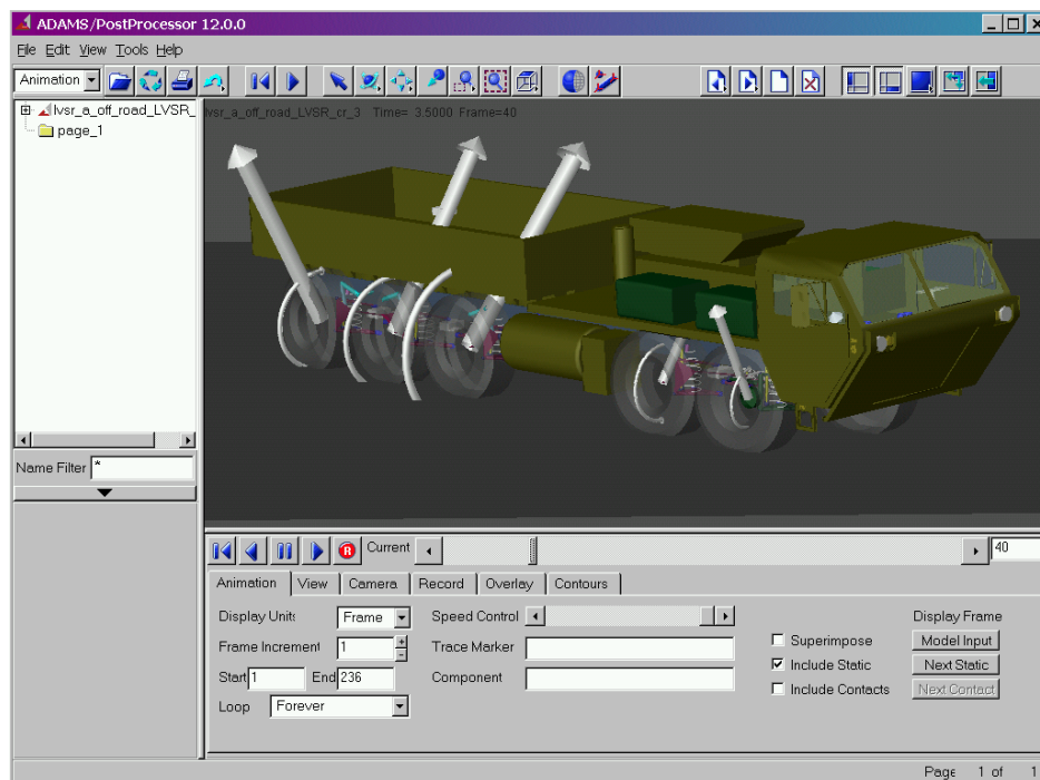
Figure E-3: Example of Graphic Simulation Results.
