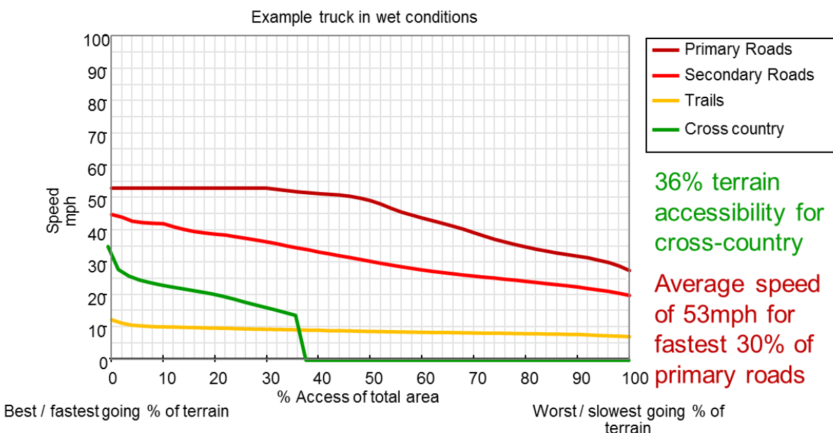
Figure 4-5: Example Cumulative Speed Curves.
