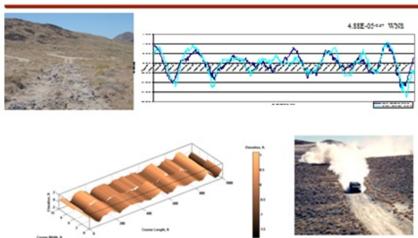
Figure E-9: Mission Profile Terrain Measurements and Vehicle Response.
