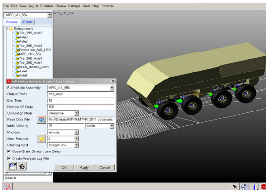
Figure 10-1: Graphical User Interface (GUI) Example. Intent is to allow a non-expert user to run simulations. Note: The dialog box contains vehicle specific fields for setting up and running a full vehicle simulation. Underlying framework is desirable to be template-based.
