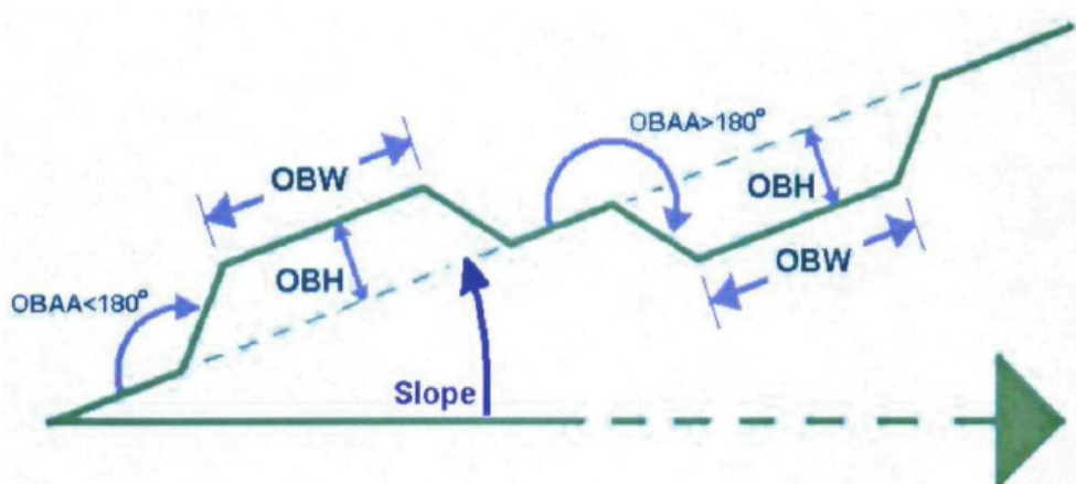
Figure 4-3: Terrain Representation.
