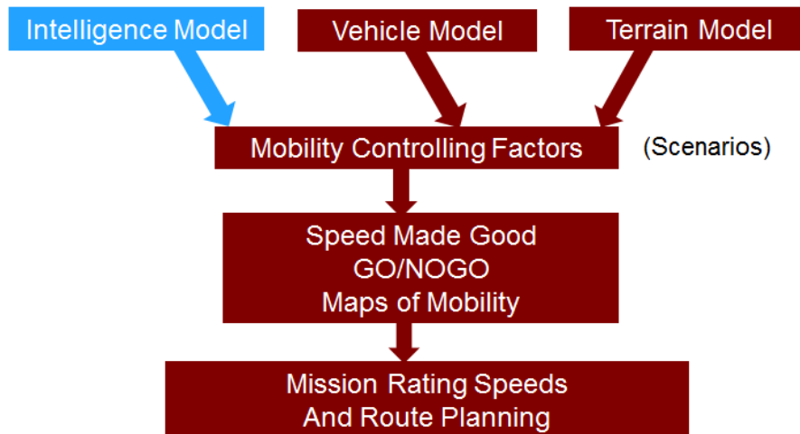
Figure 9-4: NRMM(I) Introduces Models for Vehicle Intelligence that Needs to be Included in the Prediction of Vehicle Performance.
