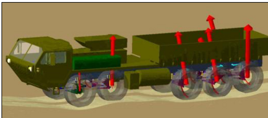
Figure F-2: LVSR-TD 10 x 10 Model During Ride Quality Simulation.
