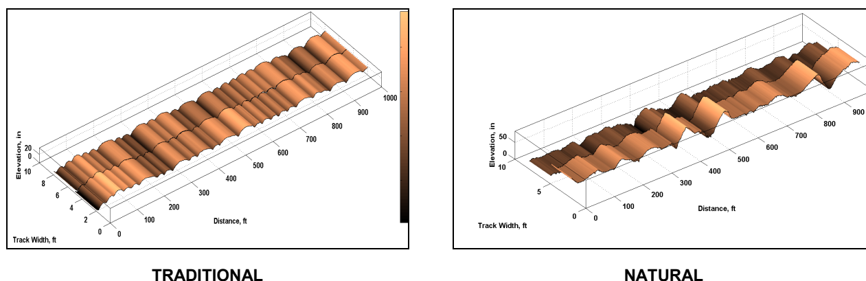
Figure F-9: Traditional RMS (In-Phase) vs. Natural WNS (Out-of-Phase) Ride Quality Courses, as Simulated.
