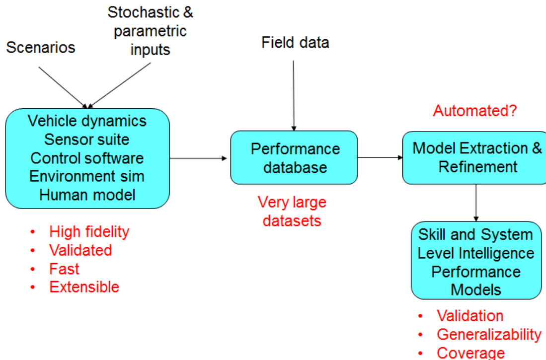
Figure 9-9: The Model Pipeline Spanning High-Fidelity Vehicle Mobility Models to Operational Vehicle Performance Models Needed by NRMM(I).
