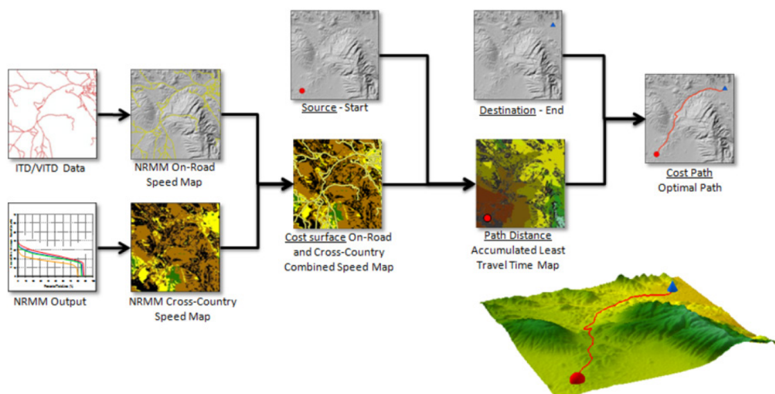
Figure 11-7: Flow Chart Outlining the Steps in the AOPM Methodology.
