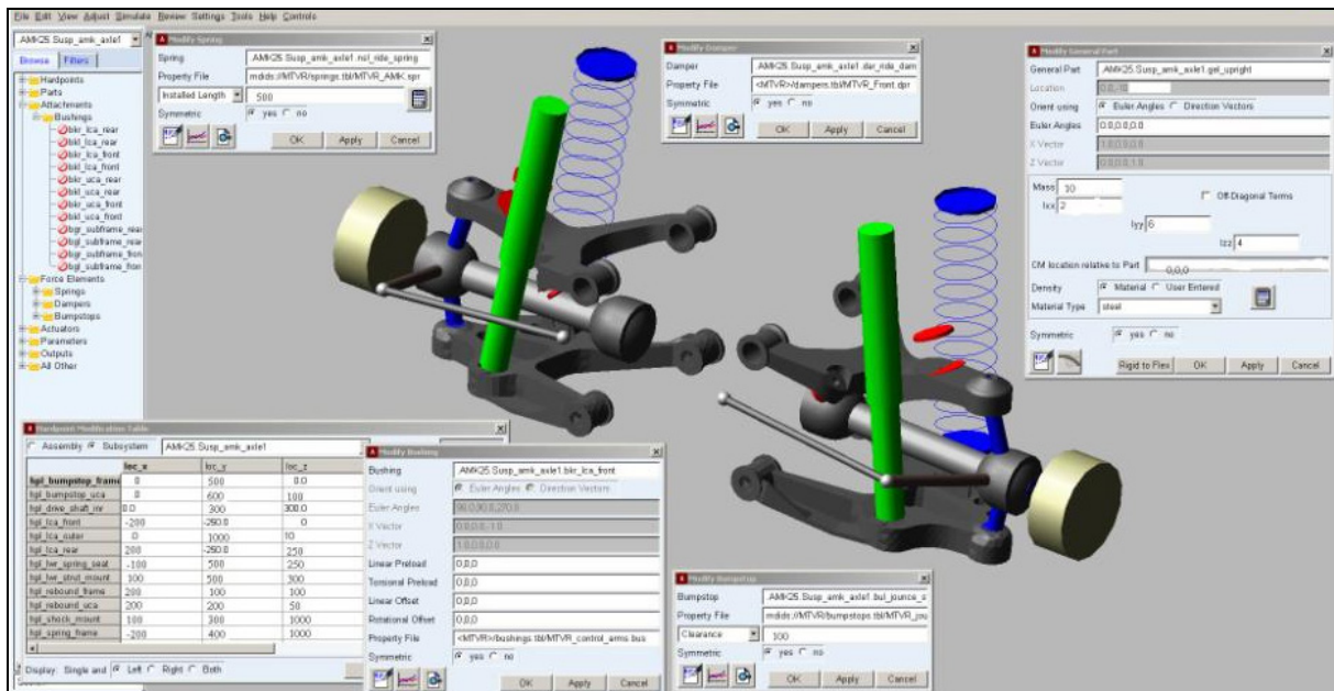
Figure F-5: Example of Geometric Data Input Through a Template.
