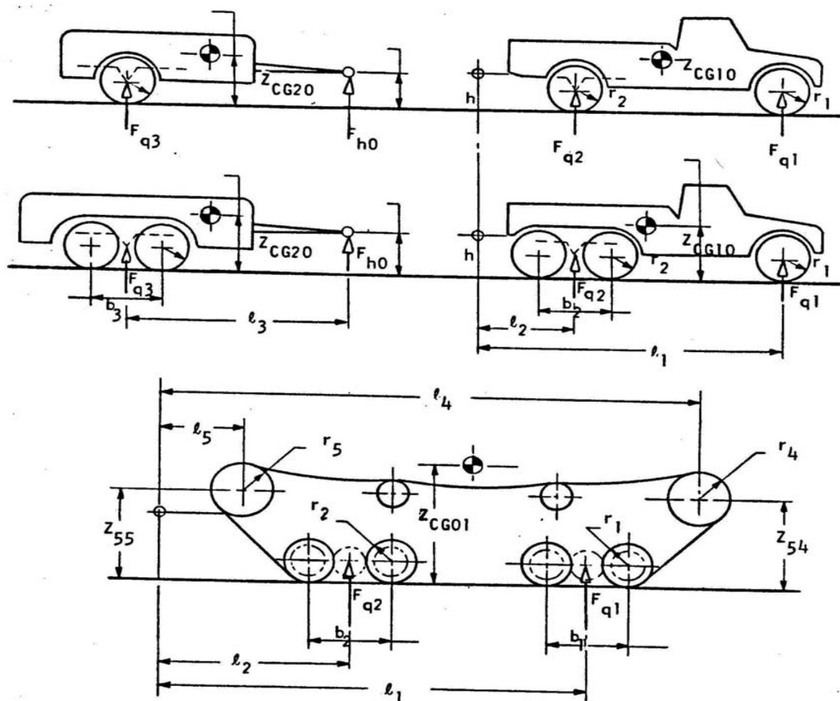
Figure 4-2: Vehicle Configurations [1].
