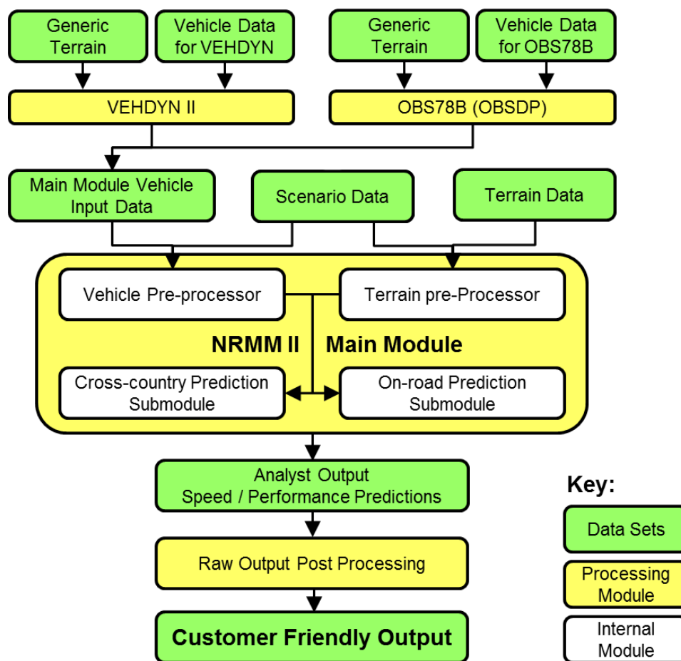
Figure 4-1: NRMM Methodology.
