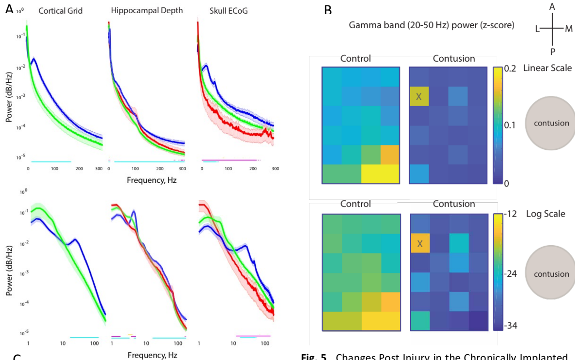
Fig. 5. Changes Post Injury in the Chronically Implanted Animals in Early Recordings. A) Wide-band power levels are significantly attenuated in the injured cortex near the contusion (Green) compared with Sham (Blue). Interestingly, this is also true on the hippocampal depth and some of the power spectrum of the rotational animal (Red) as well. A) bottom - The lower frequency bands also demonstrate the loss of power seen in the higher spectrum in the grid, and there appear to be losses in hippocampal theta (~6hz in pigs) in both injuries, although more robust in the rotational injury. The lower broadband also appears to be attenuated in the ECoG electrodes (epidural). B) The cortical grid comparing sham and control animals demonstrates significant loss of power in the gamma band (20-50Hz) at most channels in the grid, and more prominently on the side closer to the contusion (each electrode on the grid receives one square). Changes in power at higher frequencies in this penumbra of the contusion over time is one of the prominent PTE hypotheses that we will be examining, but the early response is suppression of gamma. C) Hippocampal responses to thalamic bursts are aberrant following rotation injury (*).
